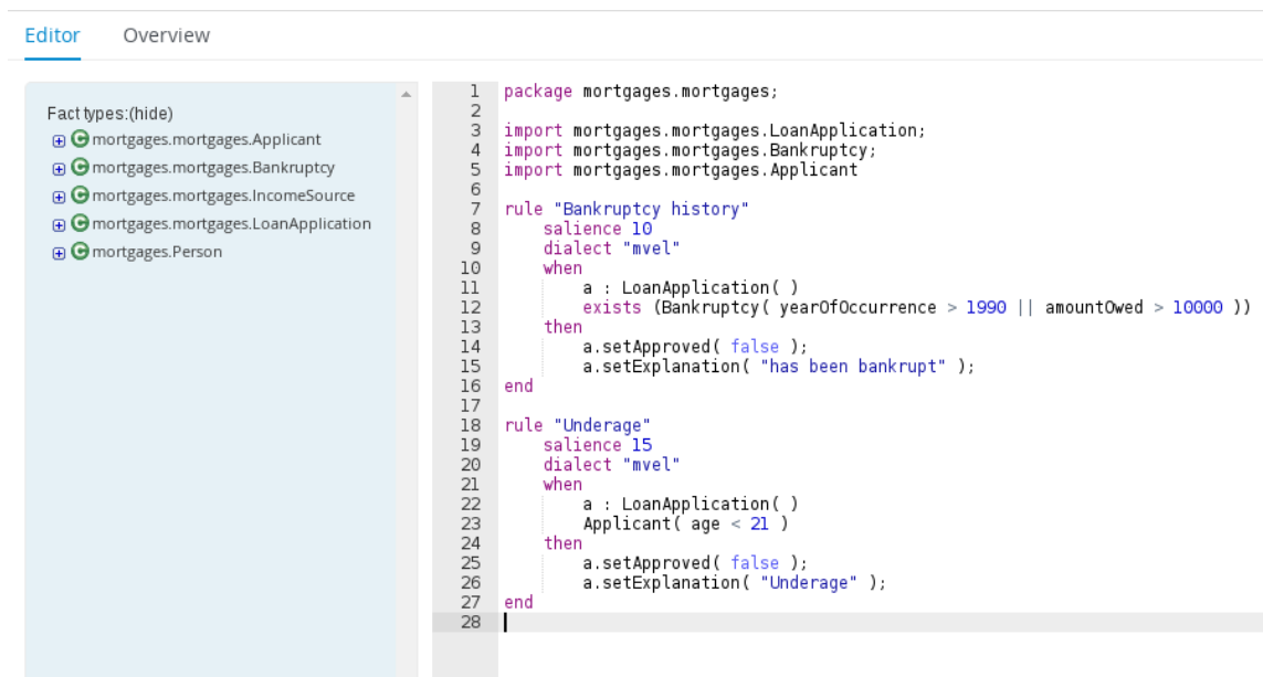
Figure 4.1. Sample DRL file with required components and optional rule attributes
