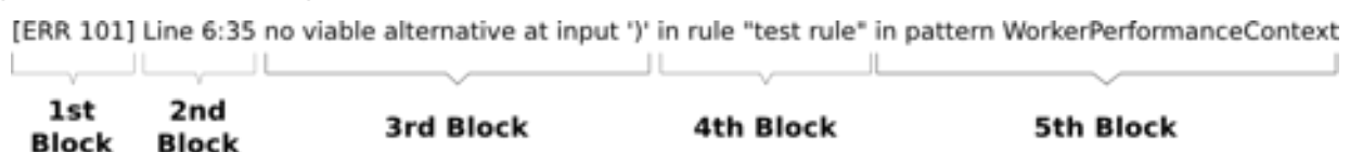
Figure 16.1. Error message format for DRL file problems
