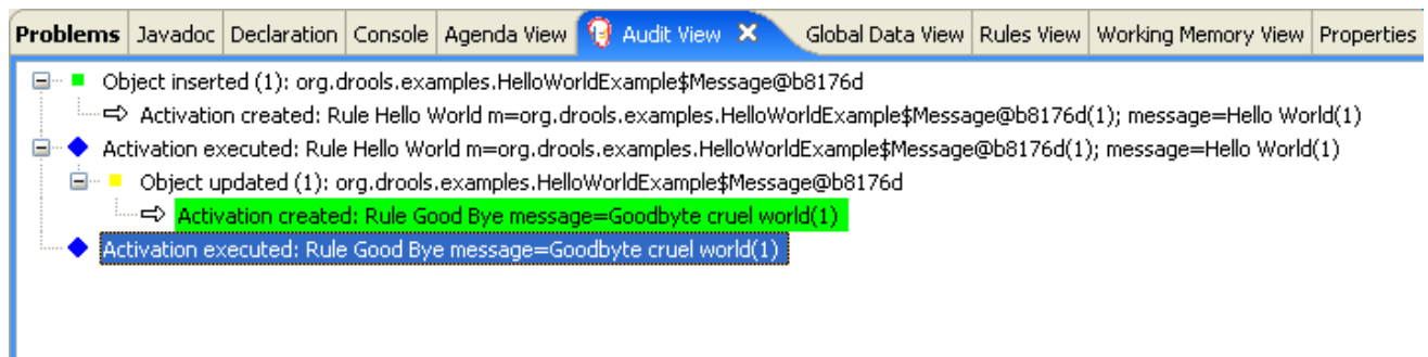
Figure 88.3. Hello World example Audit View
