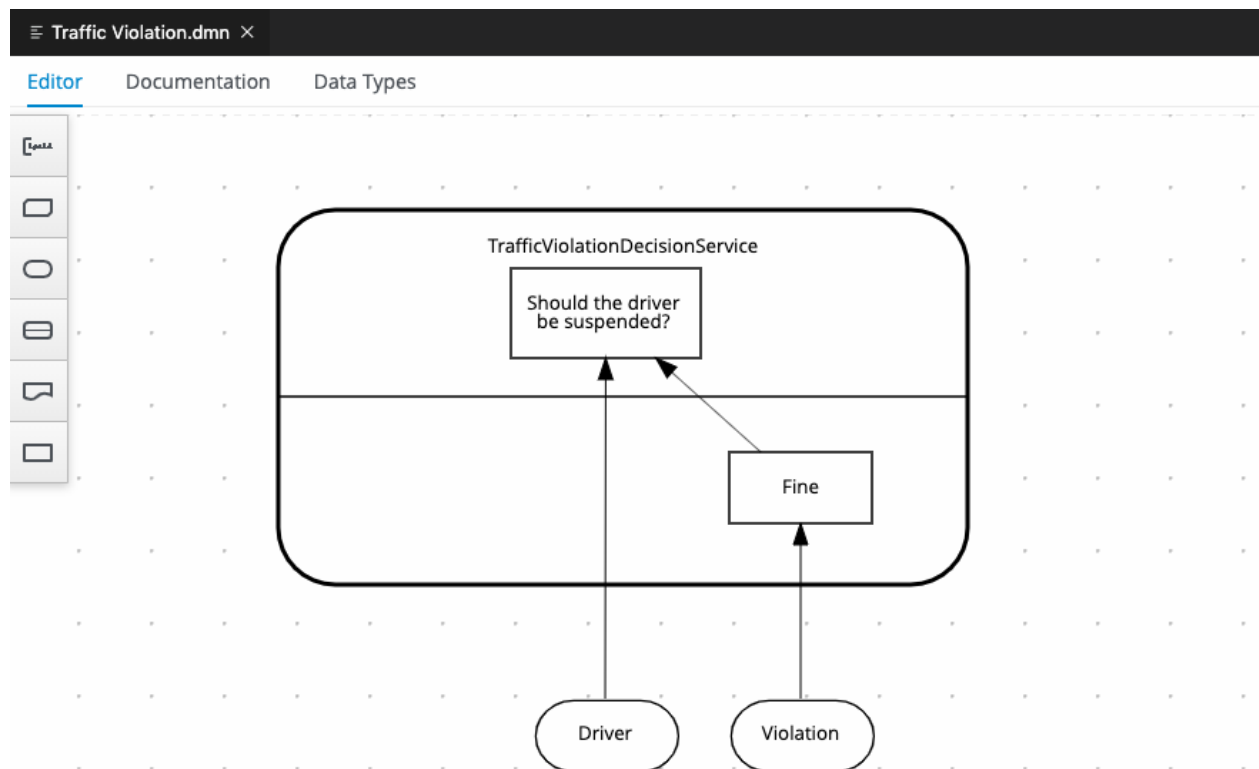
Figure 7.1. Example TrafficViolationDecisionService decision service with single-output decision
