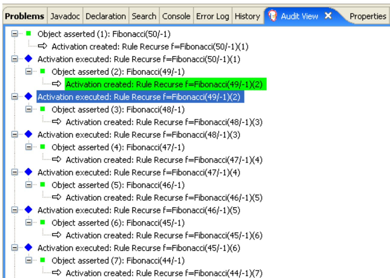
Figure 21.7. Rule "Recurse" in Audit View
