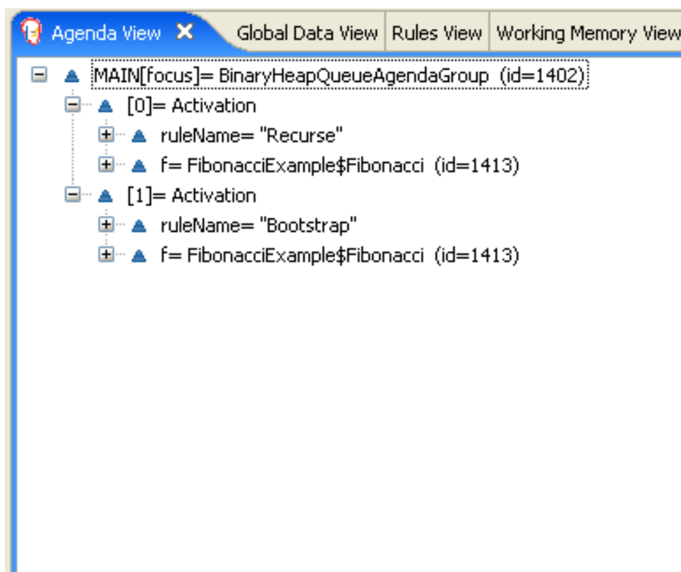
Figure 88.8. Rules "Recurse" and "Bootstrap" in Agenda View 1
