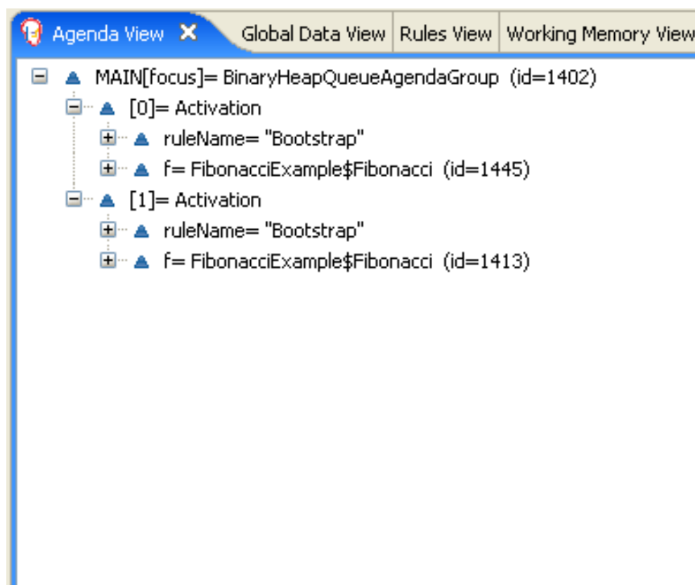
Figure 88.9. Rules "Recurse" and "Bootstrap" in Agenda View 2
