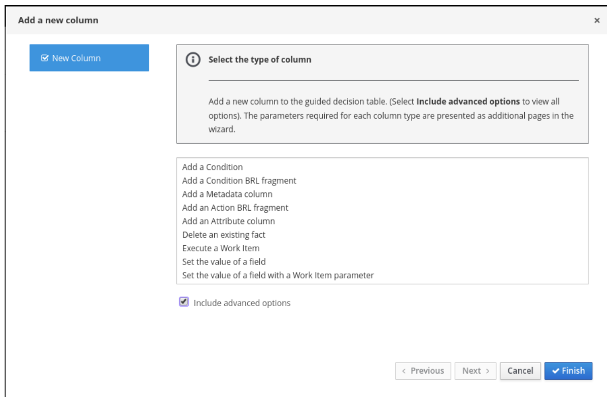
Figure 29.1. Add columns
