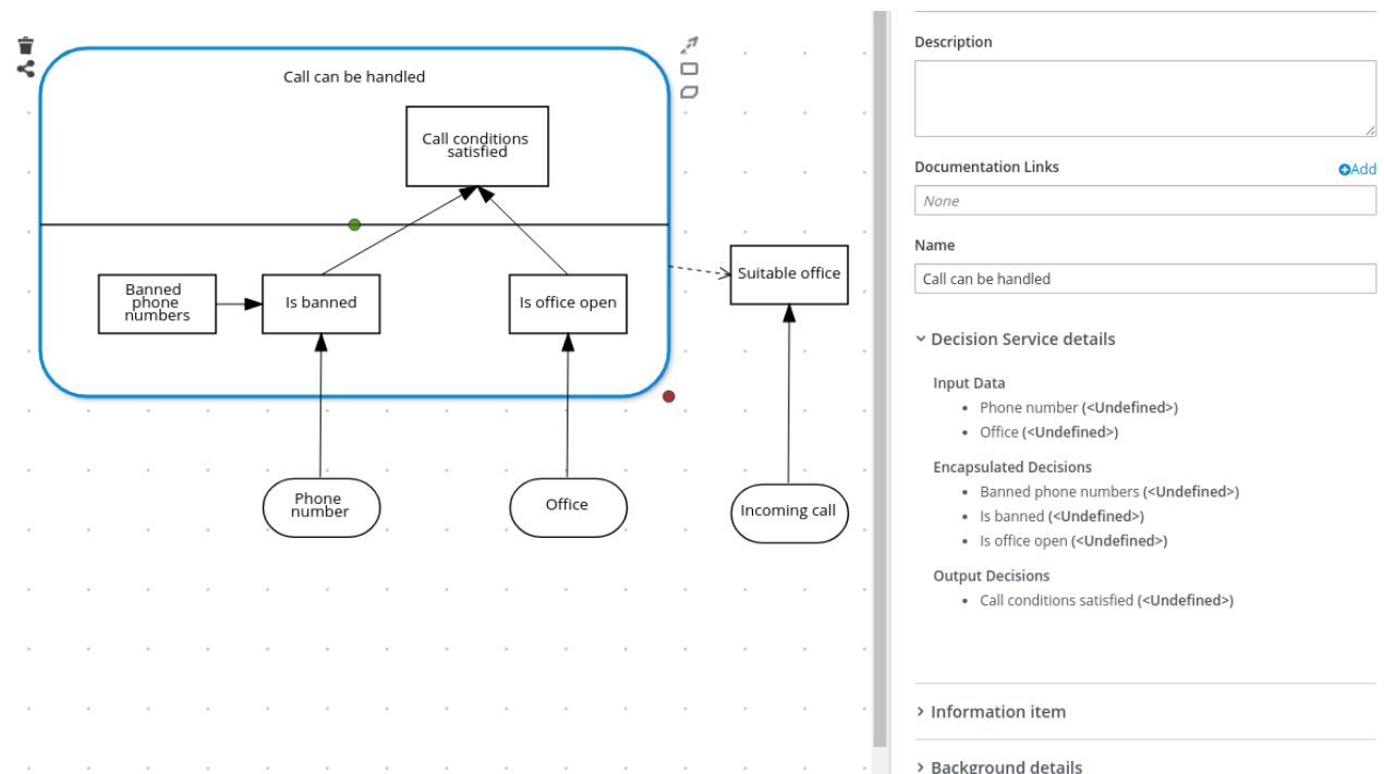
Figure 6.65. Decision Service details
