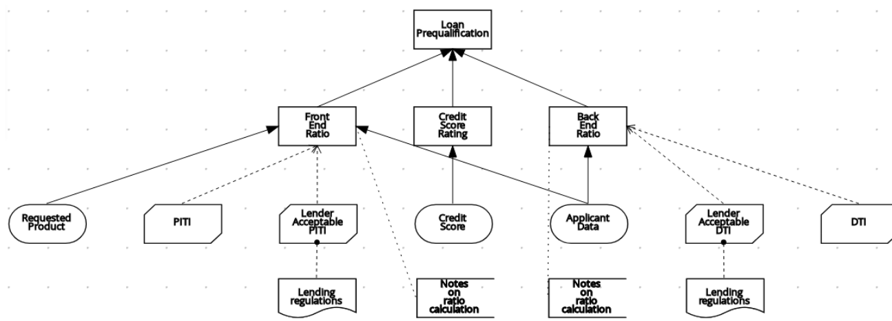
Figure 4.1. Example DRD: Loan prequalification
