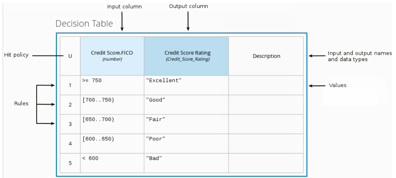
Figure 4.3. Decision table for credit score rating
