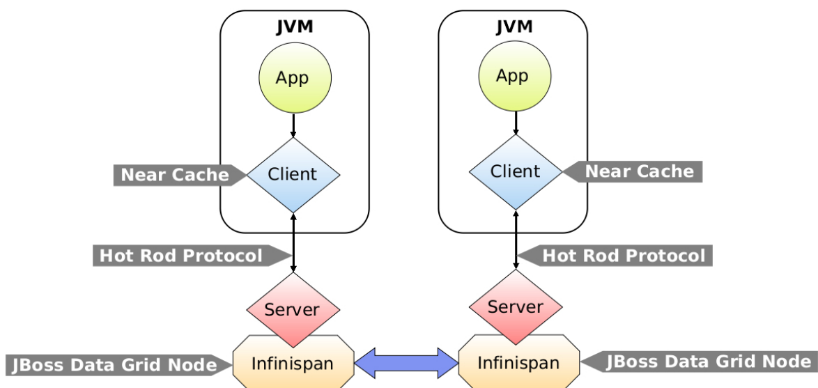
Figure 40.1. Near Caching Architecture
