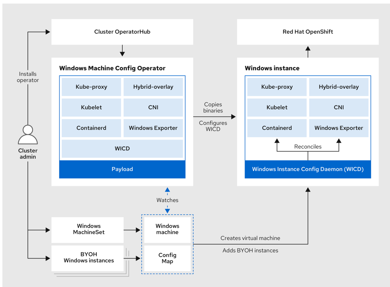
Figure 3.1. WMCO design
