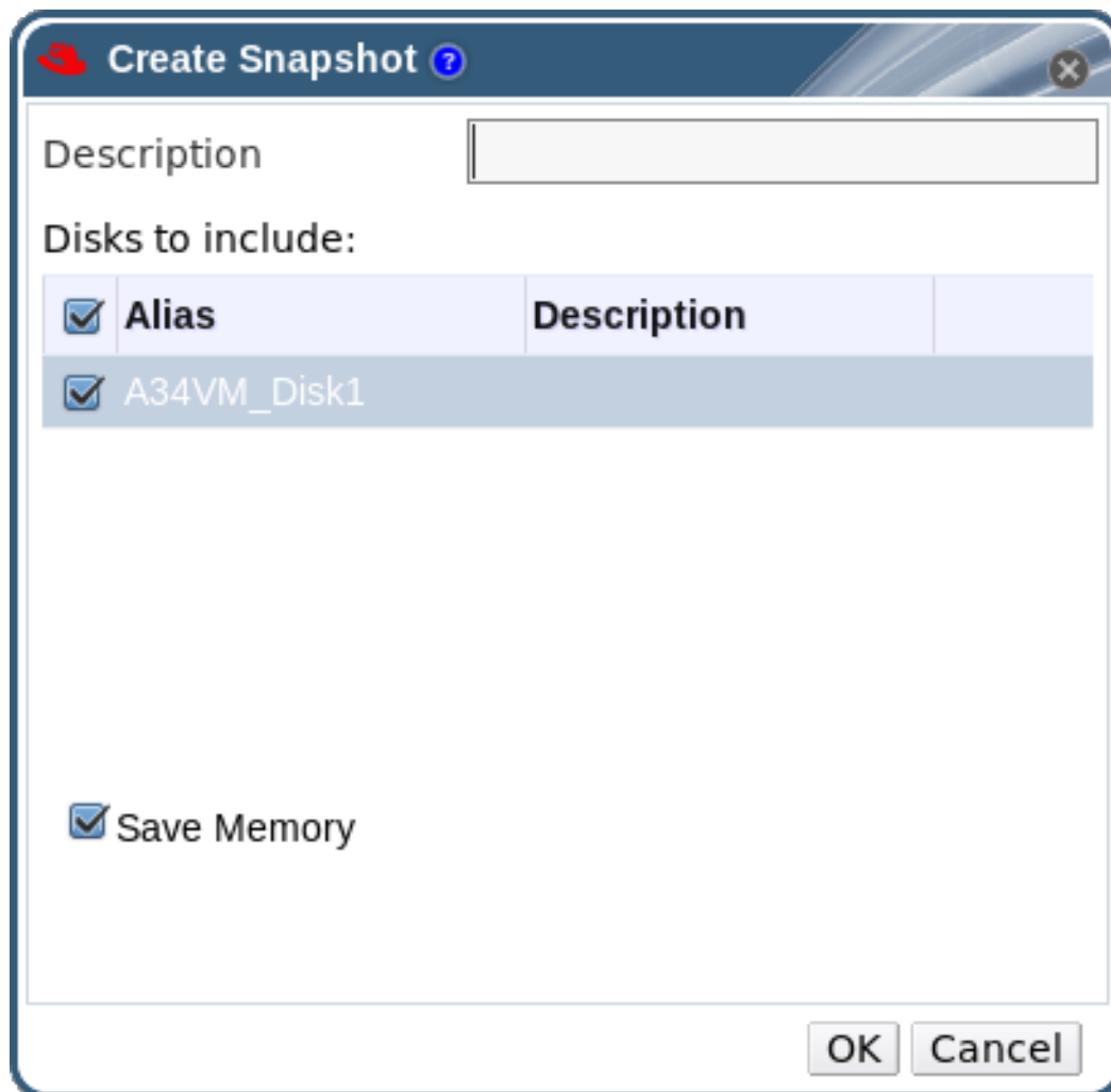
Figure 6.1. Create snapshot
