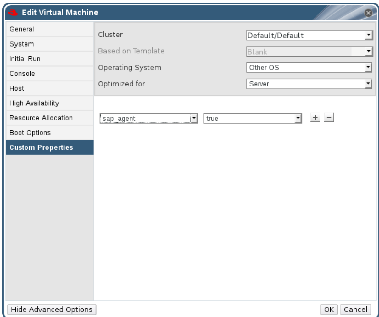
Figure 6.13. Enable SAP
