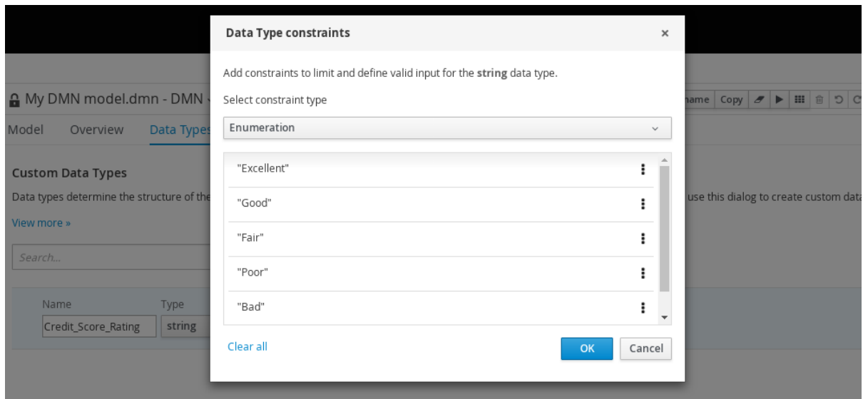
Figure 3.17. Adding constraints to the new data type
