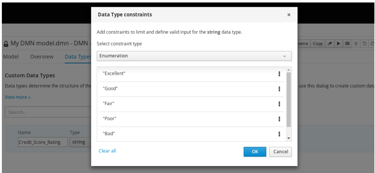
Figure 3.27. Adding constraints to the new data type
