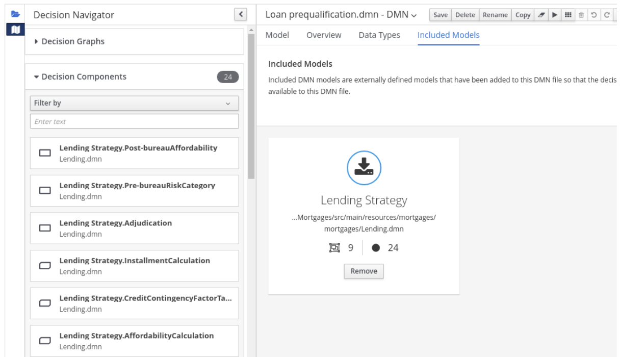
Figure 3.37. DMN file with decision components from the included DMN model
