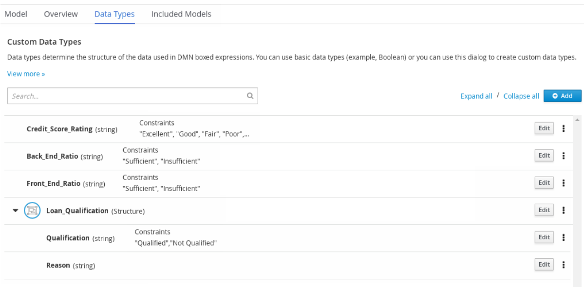
Figure 3.31. Adding nested data types with constraints
