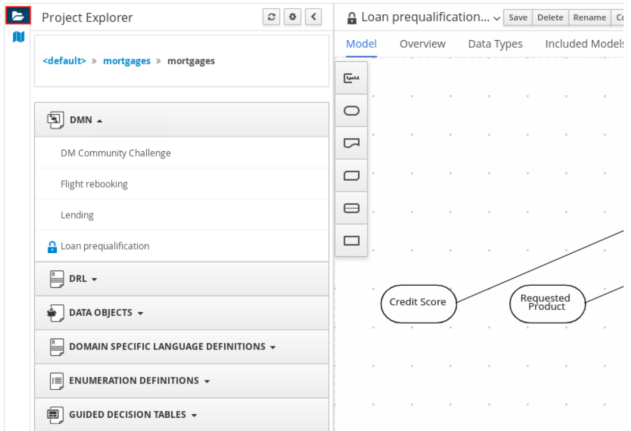
Figure 3.40. Project Explorer view
