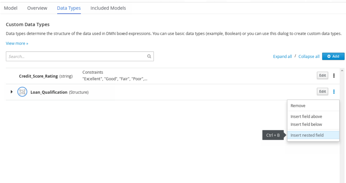
Figure 3.30. Adding a new structured data type with nested fields
