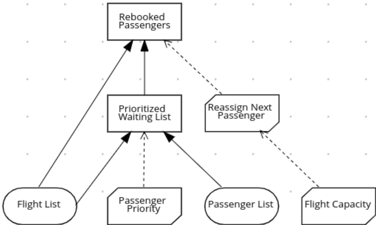
Figure 1.16. DRD for flight rebooking
