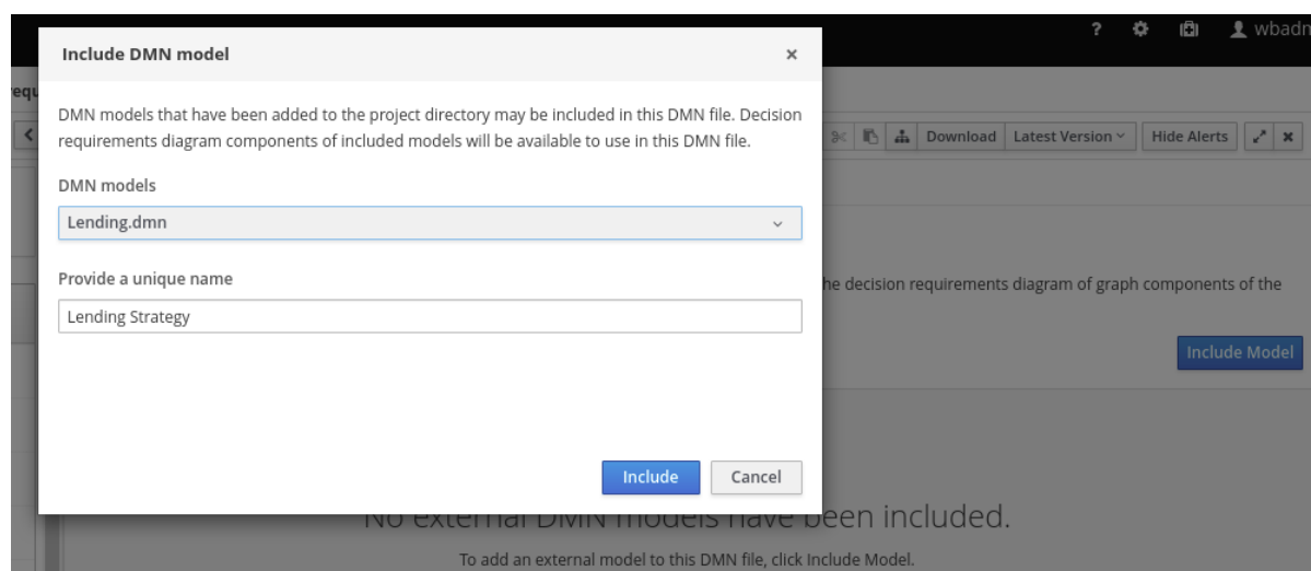
Figure 3.36. Including a DMN model
