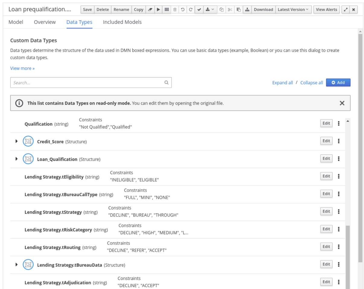
Figure 3.38. DMN file with data types from the included DMN model
