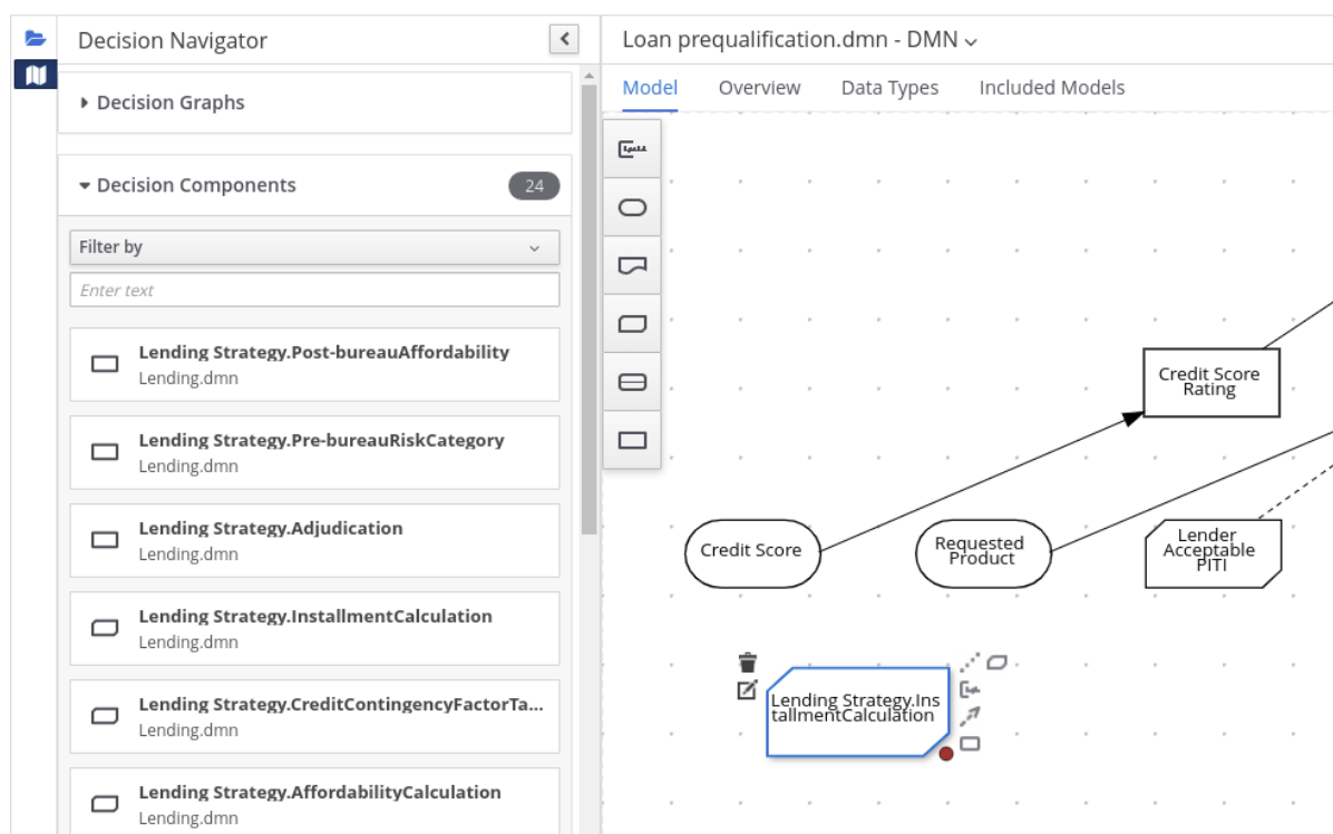
Figure 3.39. Adding DRD components from the included DMN model
