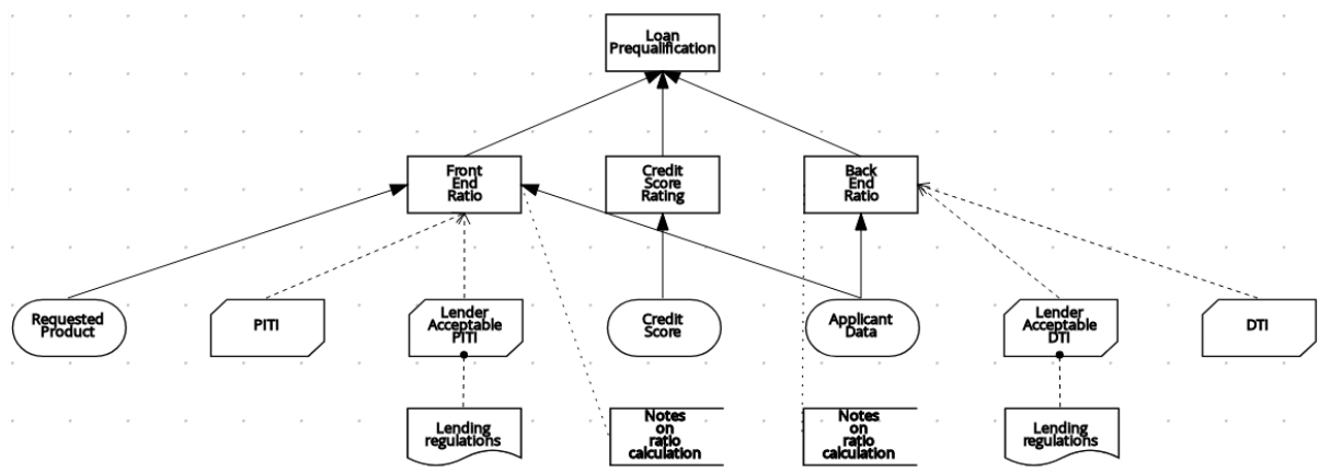
Figure 3.9. Completed DRD for loan prequalification
