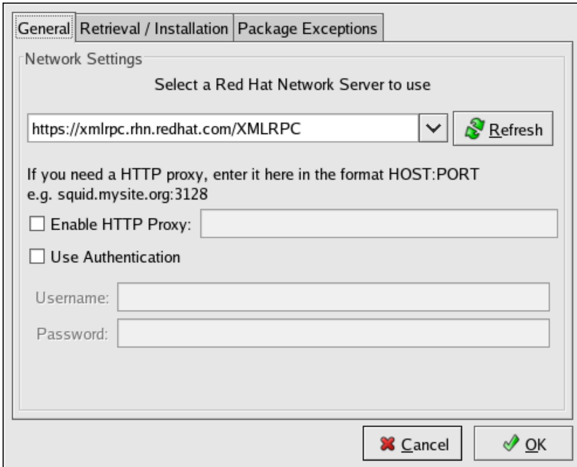
Figure 2.16. General Settings
