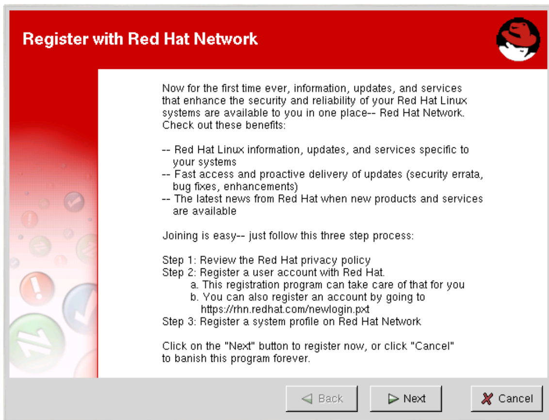
Figure 5.4. Welcome Screen
