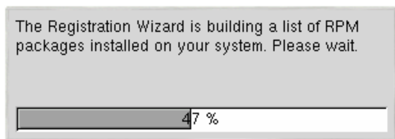
Figure 5.9. Registration Wizard
