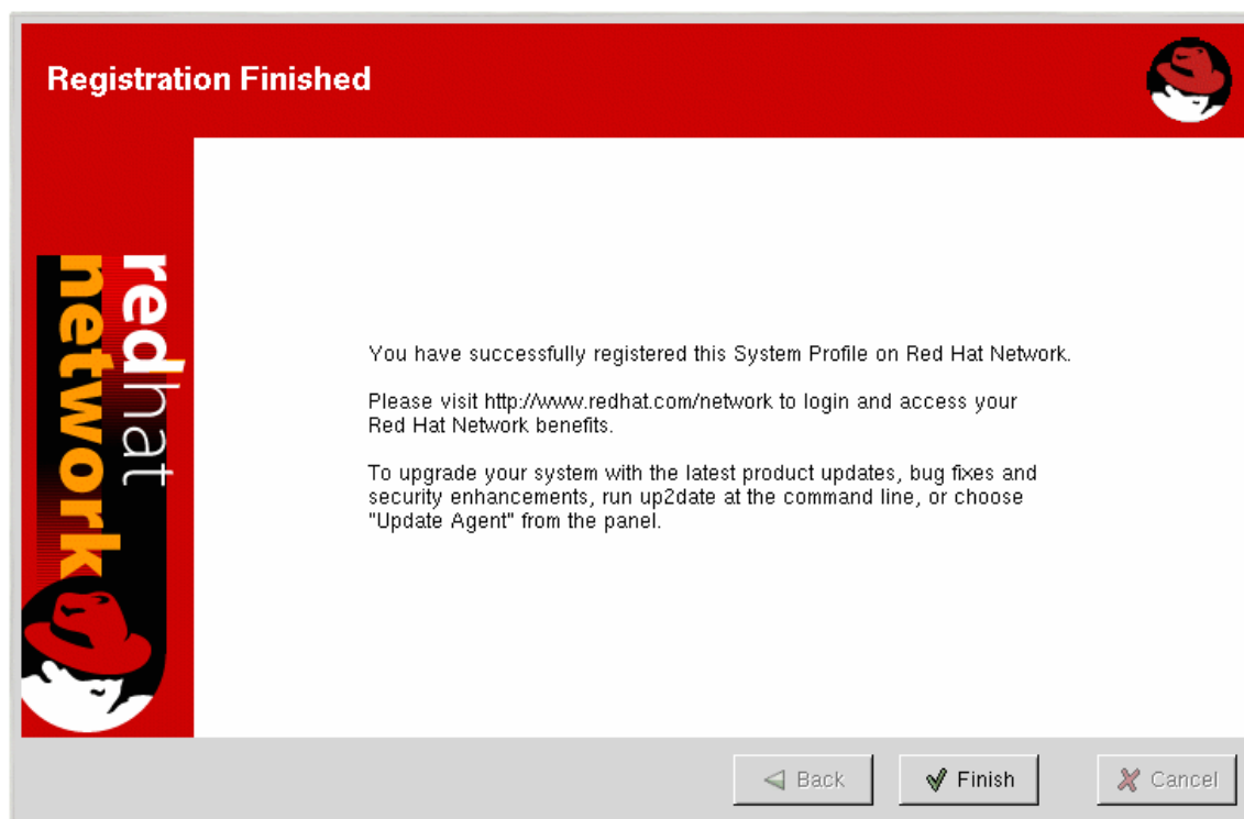
Figure 5.14. Registration Finished
