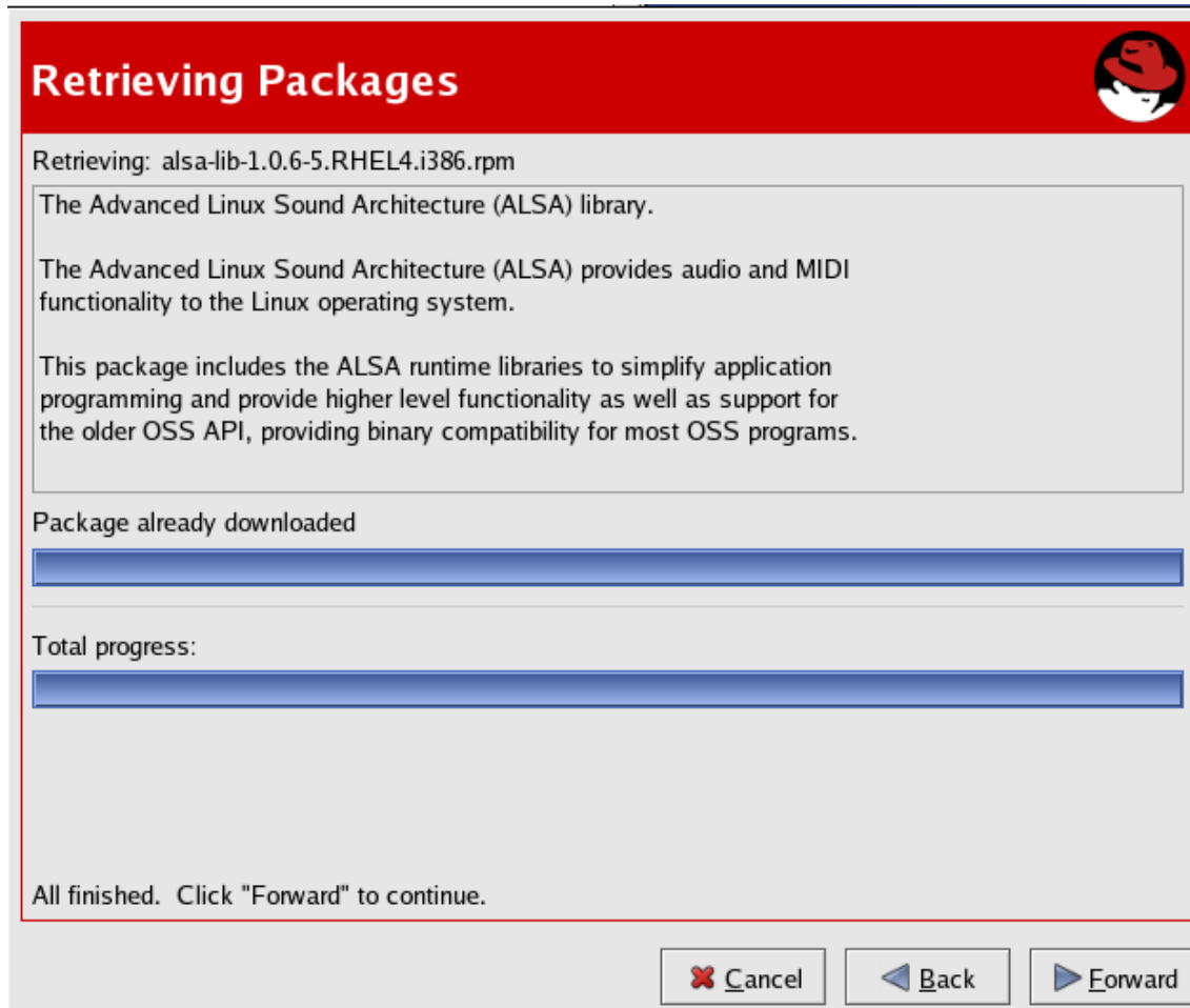
Figure 2.13. Retrieving Packages
