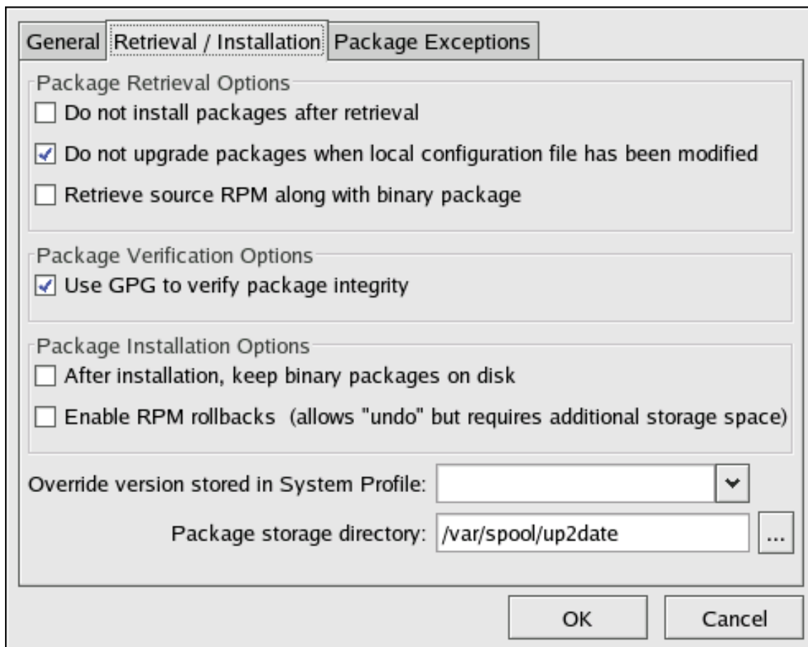
Figure 2.17. Retrieval/Installation Settings
