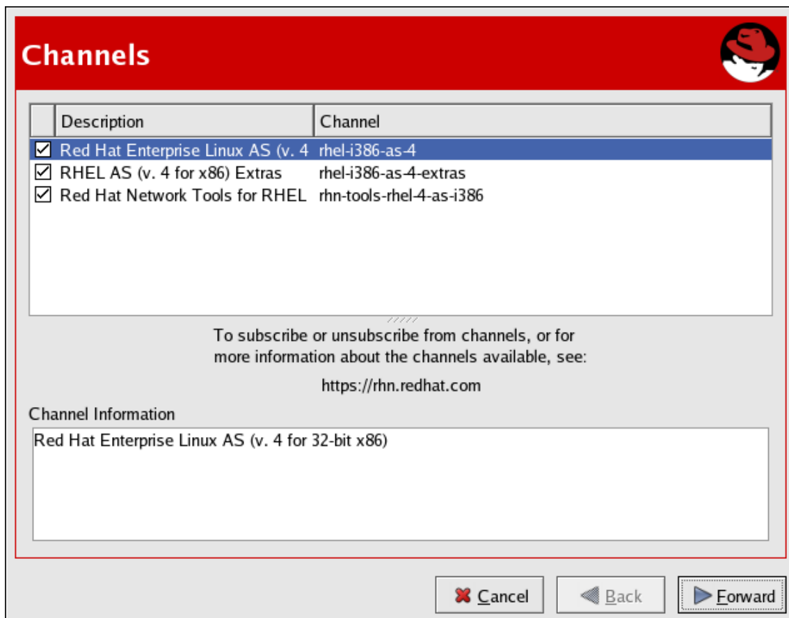
Figure 2.8. Channels
