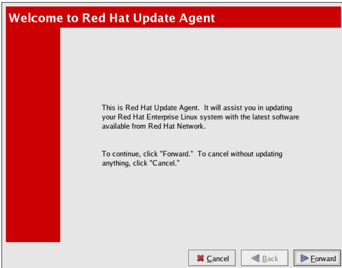
Figure 2.3. Welcome Screen
