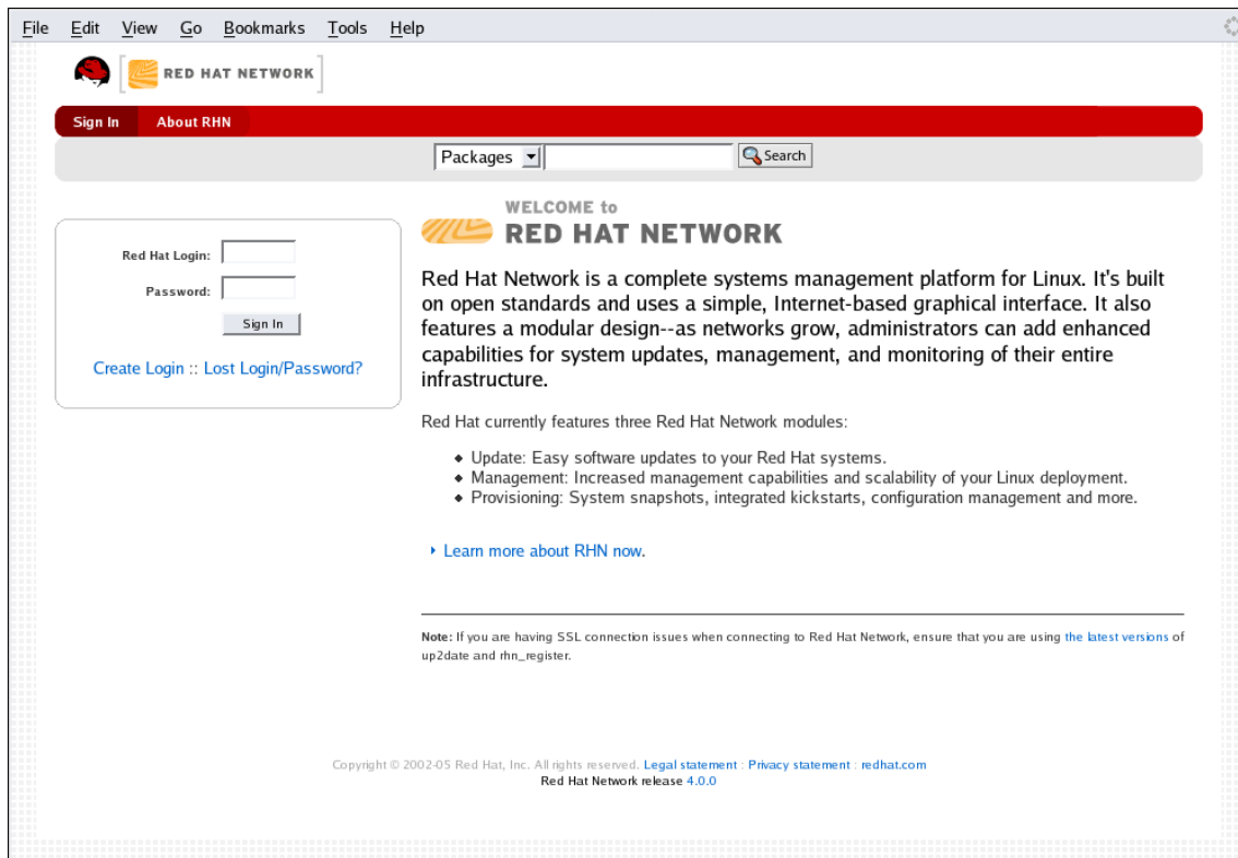
Figure 6.4. RHN Website
