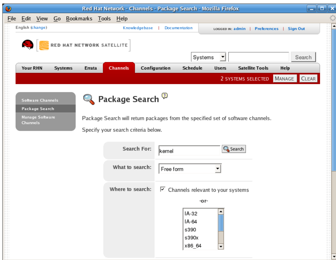
Figure 6.17. Package Search
