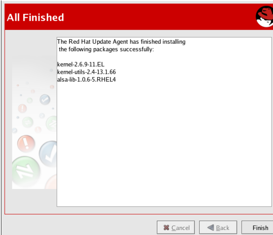
Figure 2.15. All Finished
