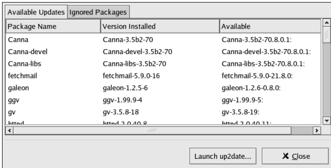
Figure 4.3. Available Updates
