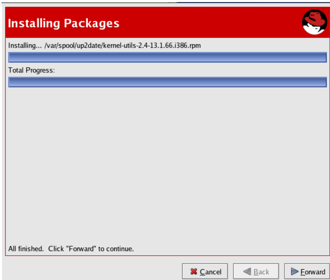
Figure 2.14. Installing Packages
