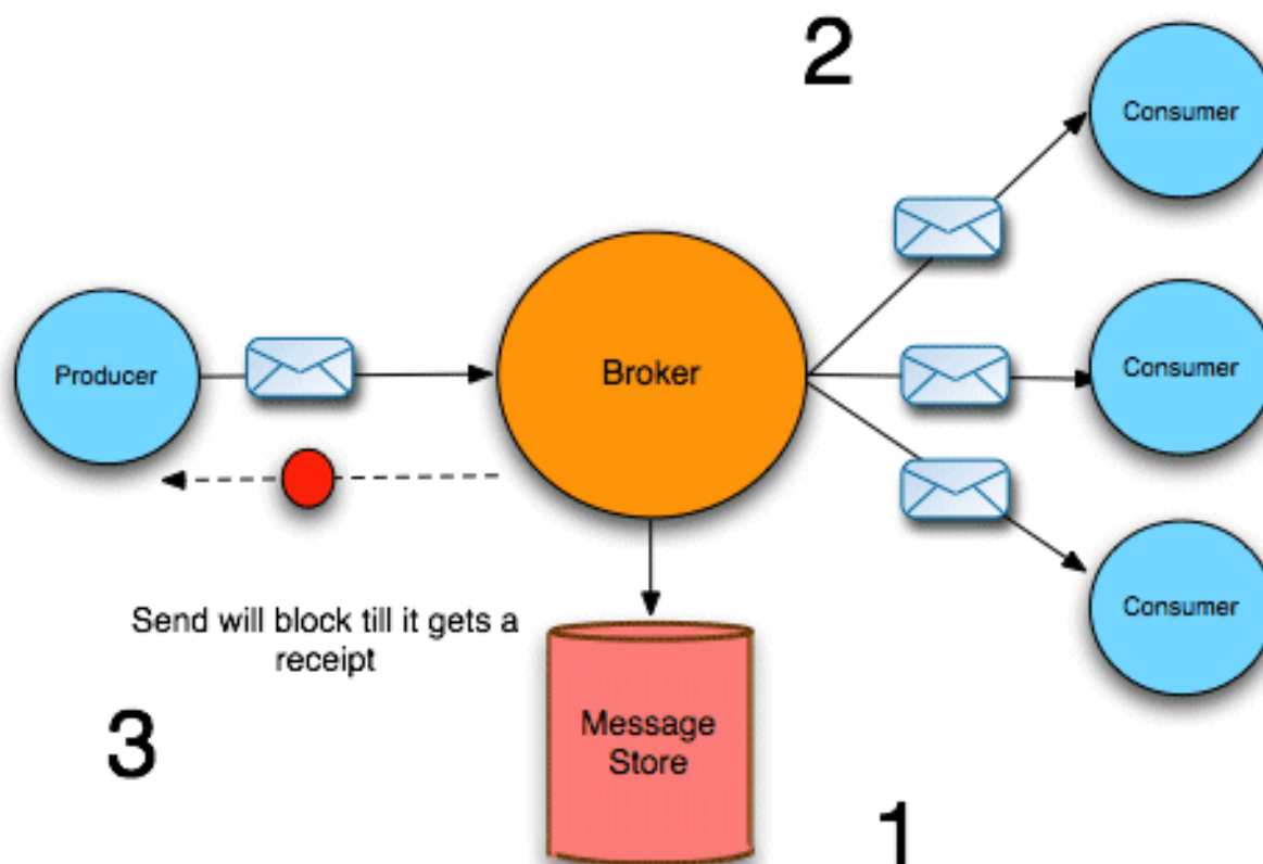
Figure 6.1. Synchronous Dispatch through a Persistent Broker
