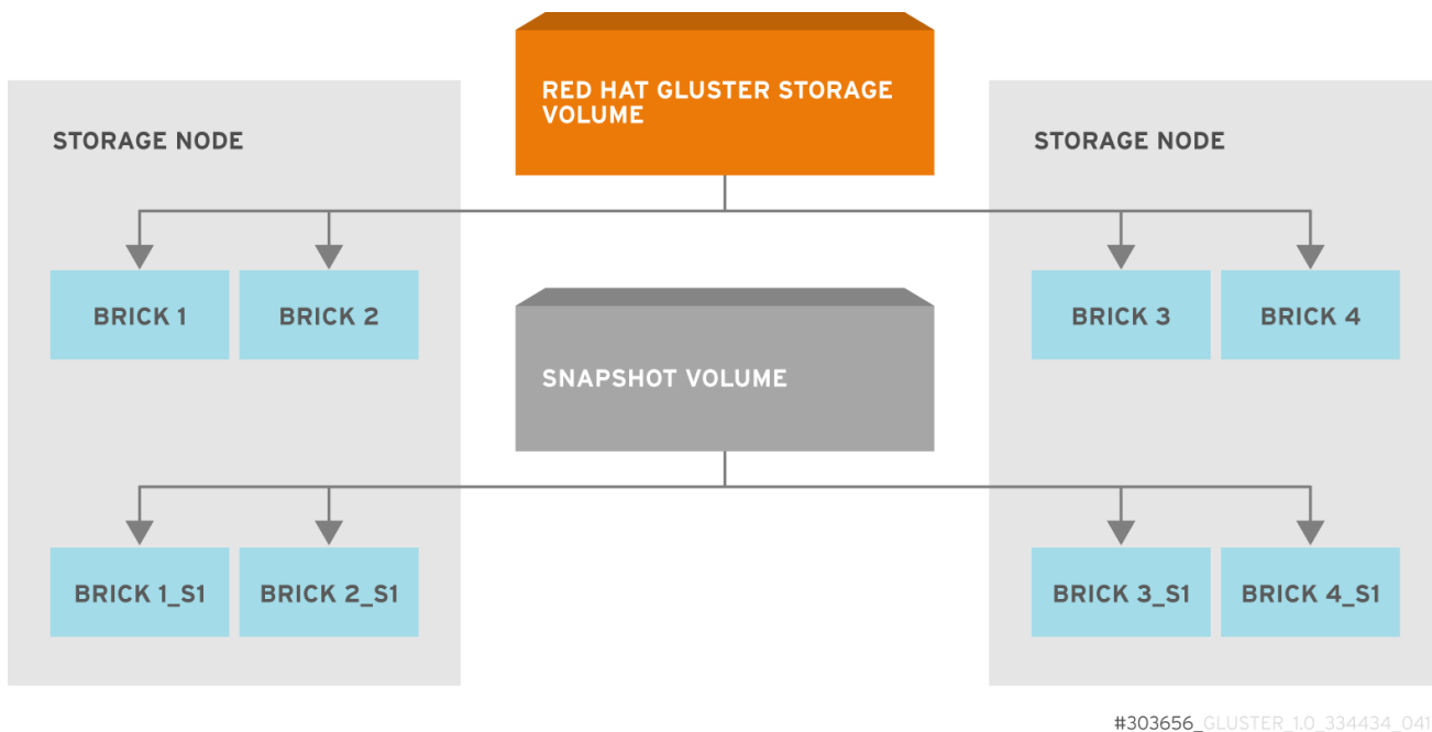
Figure 8.1. Snapshot Architecture
