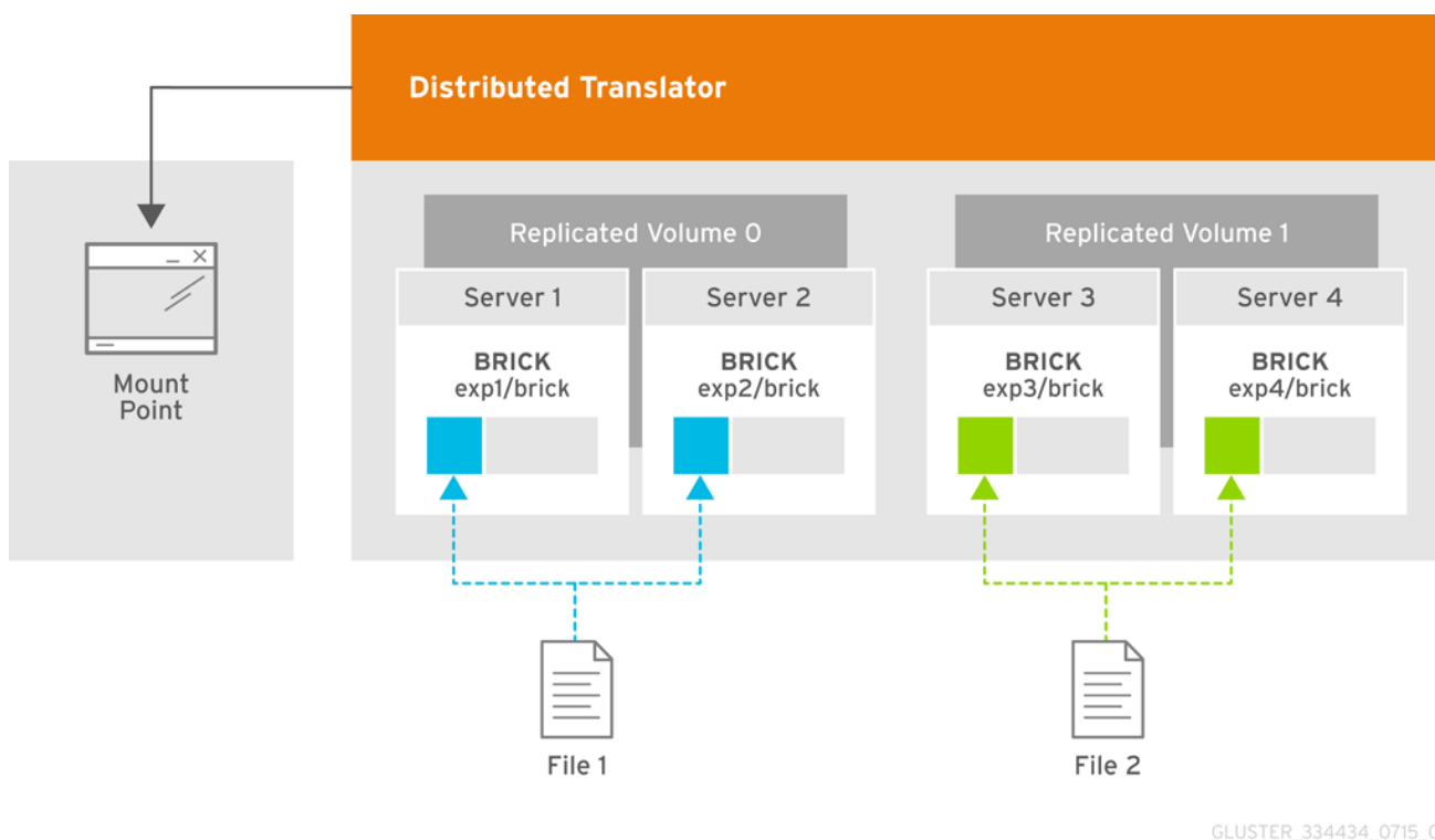
Figure 5.5. Illustration of a Two-way Distributed Replicated Volume
