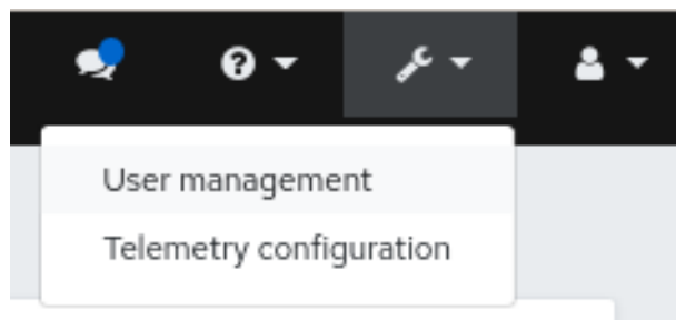
Figure 2.8. User management
