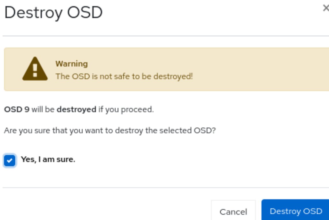
Figure 11.12. Destroying OSDs
