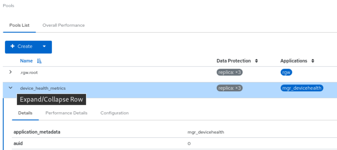
Figure 6.9. Monitoring pools
