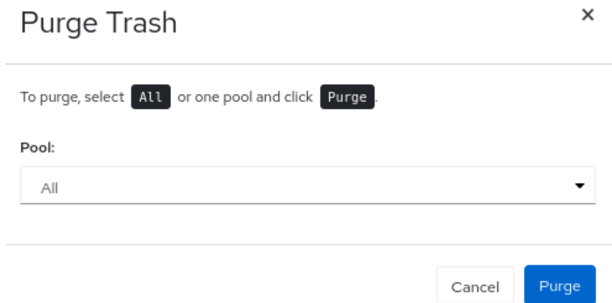
Figure 13.6. Purge trash
