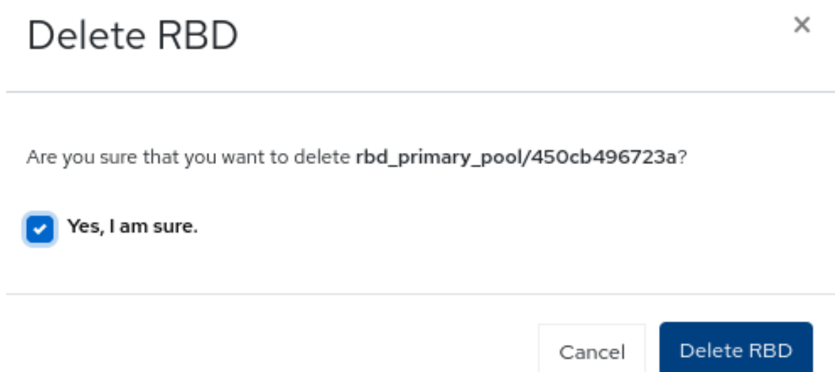
Figure 13.8. Deleting images
