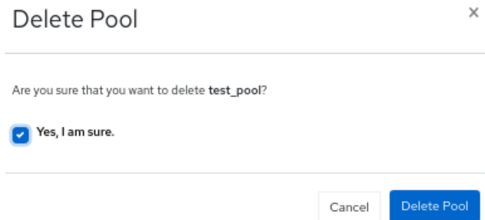
Figure 9.4. Delete pools
