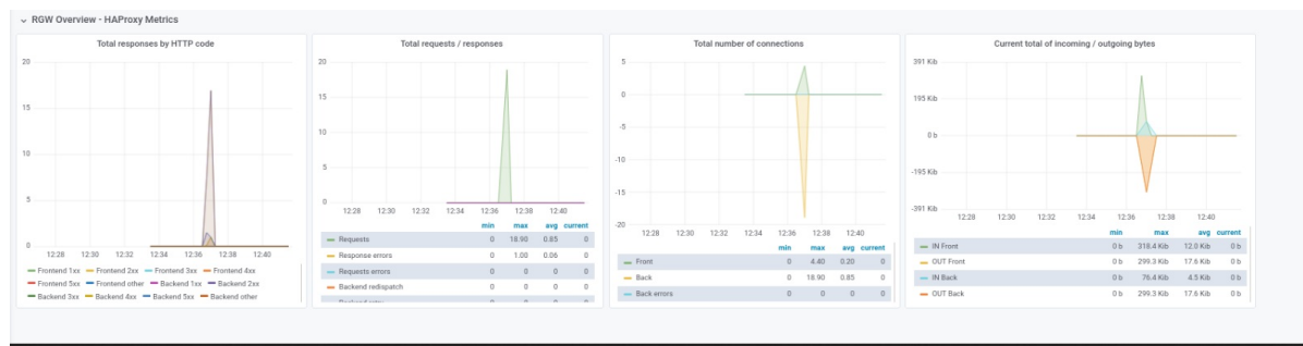
Figure 6.6. HAProxy metrics
