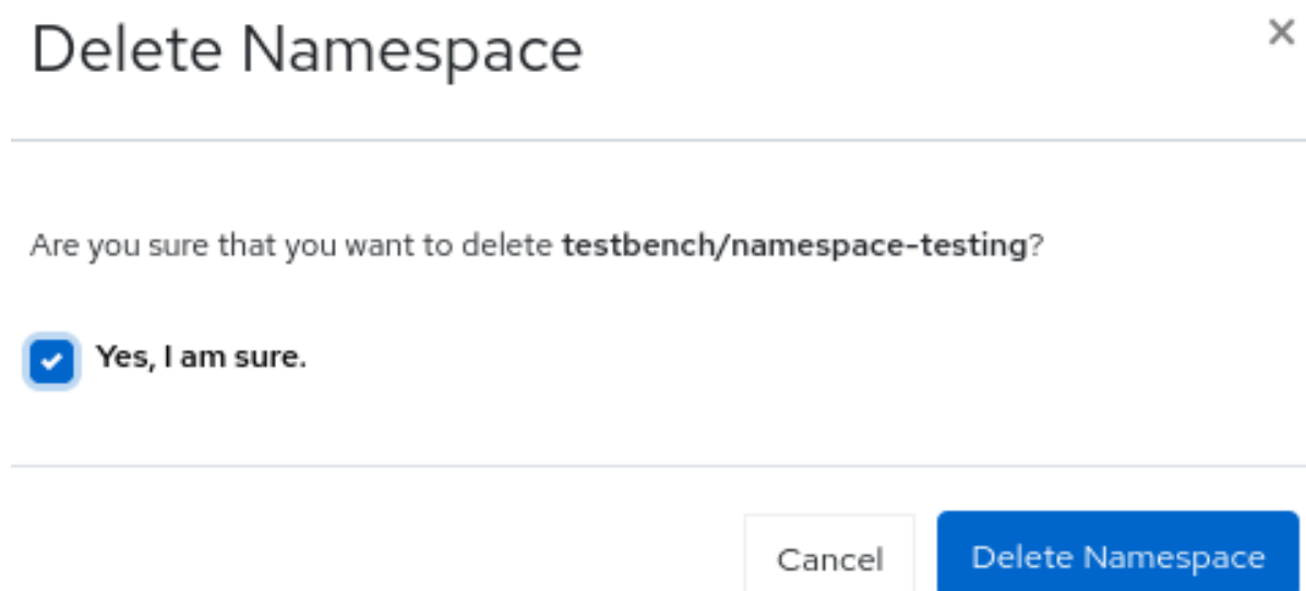
Figure 13.9. Deleting namespaces
