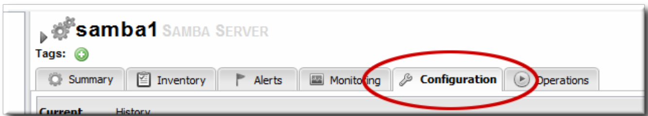
Figure 2. Configuration Tab
