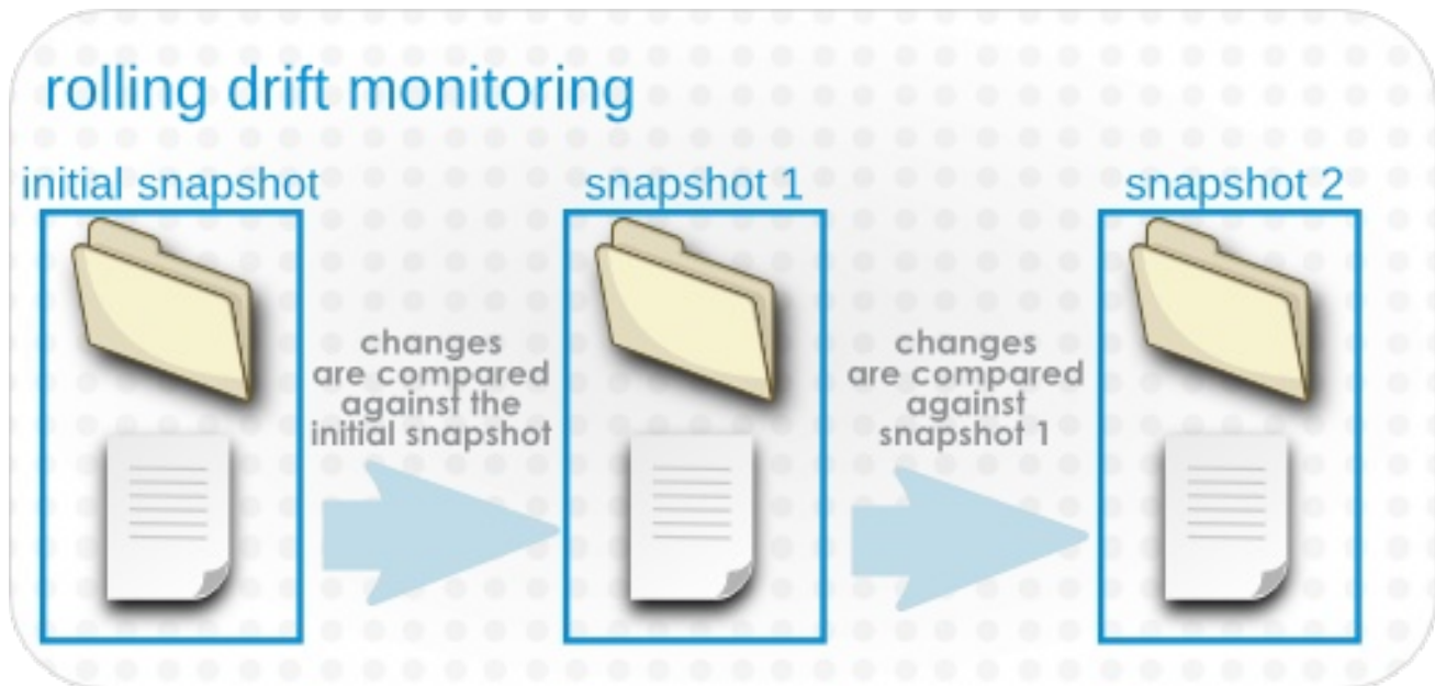
Figure 3. Rolling Snapshots
