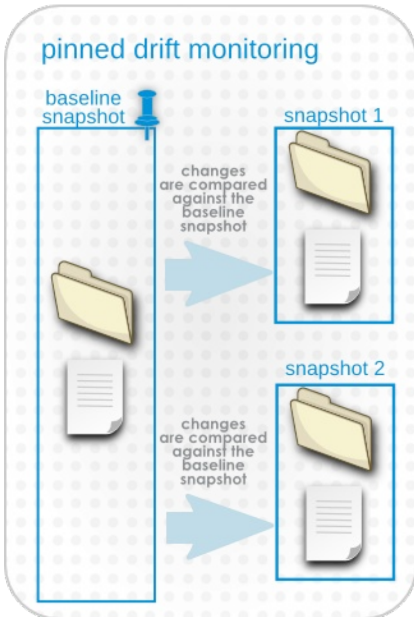
Figure 4. Pinned Snapshots
