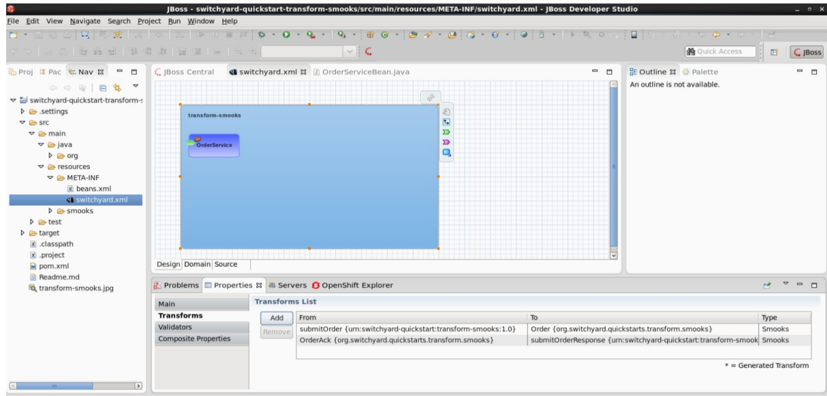
Figure 11.1. Smooks Transformations in SwitchYard Editor
