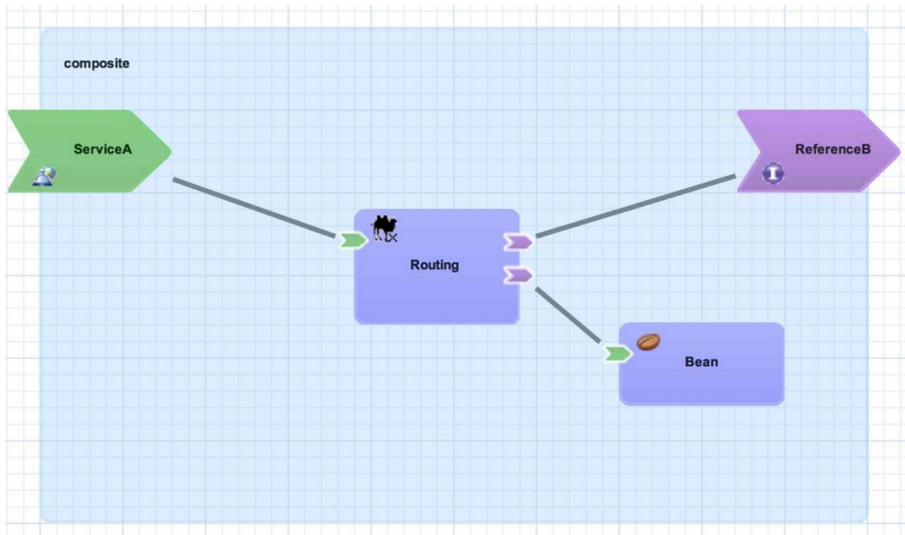
Figure 4.1. Composite
