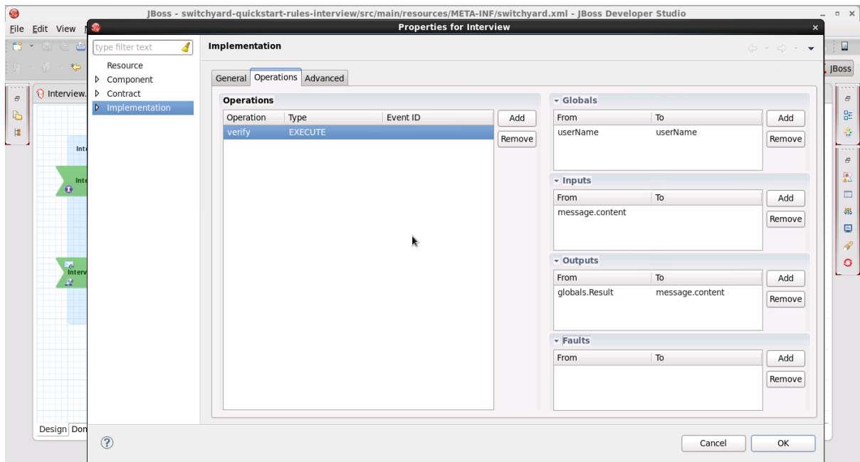
Figure 9.4. Operations Mapping
