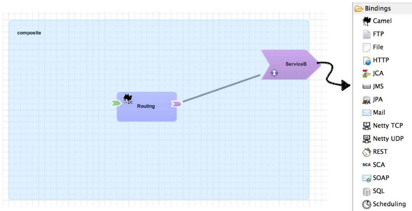
Figure 4.10. Reference Bindings
