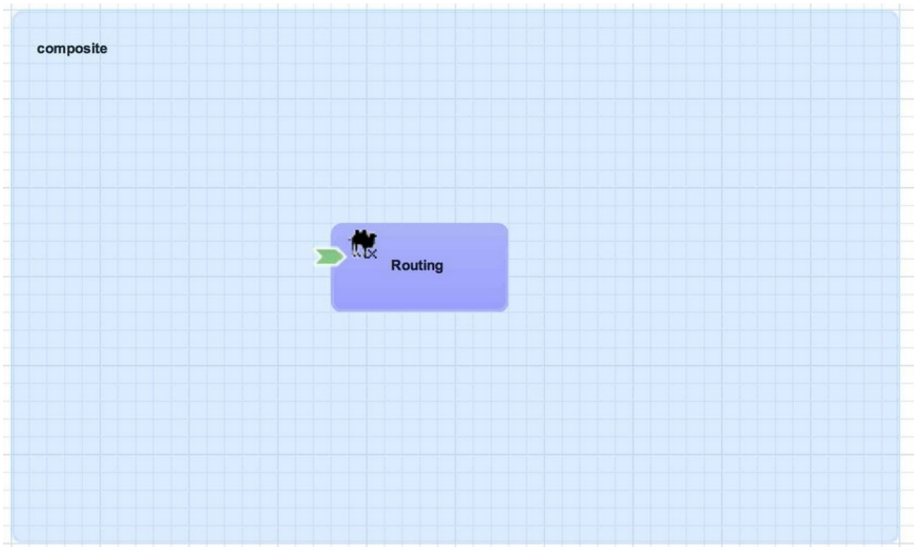
Figure 4.5. Component Service
