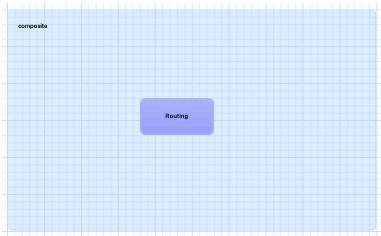
Figure 4.3. Component
