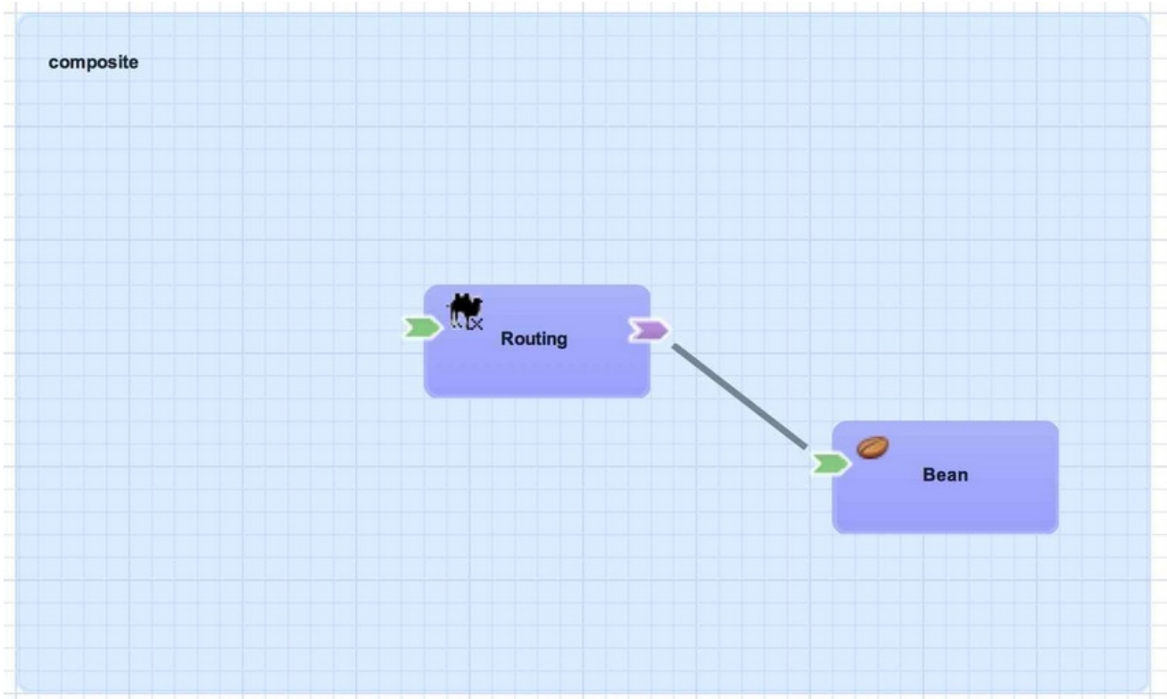
Figure 4.9. Composite Reference
