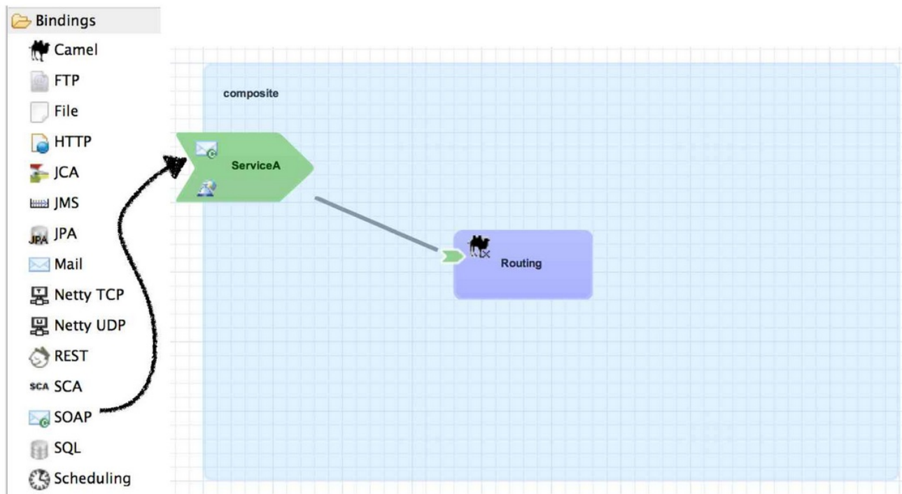
Figure 4.7. Service Binding
