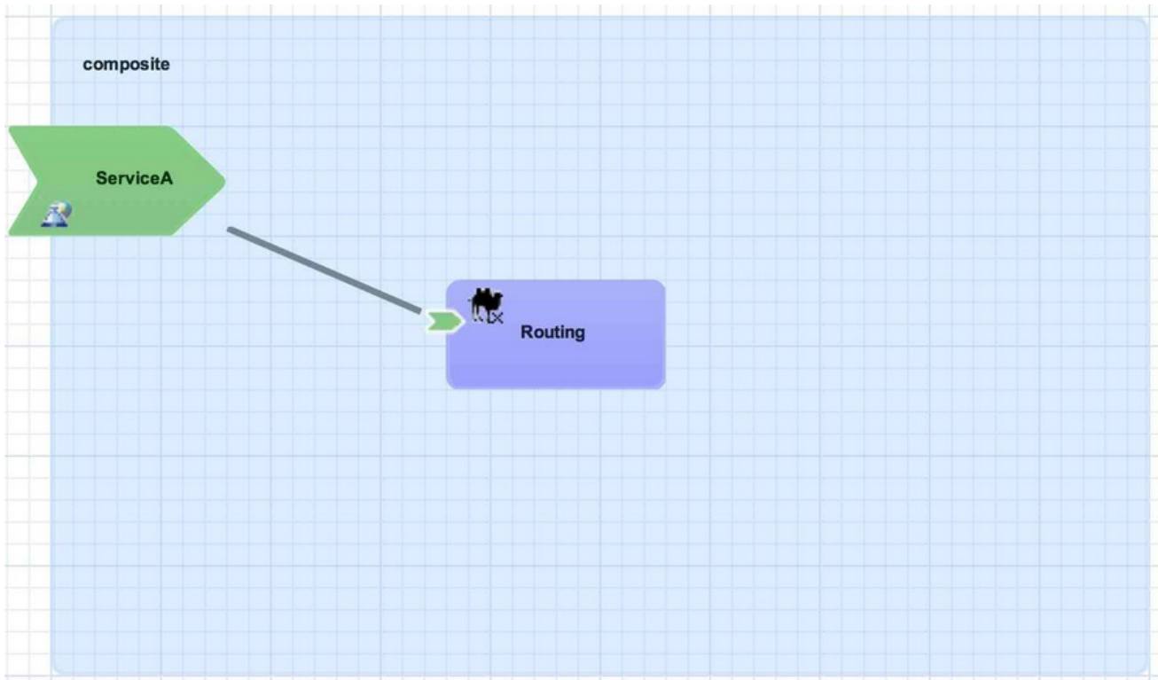
Figure 4.6. Composite Service
