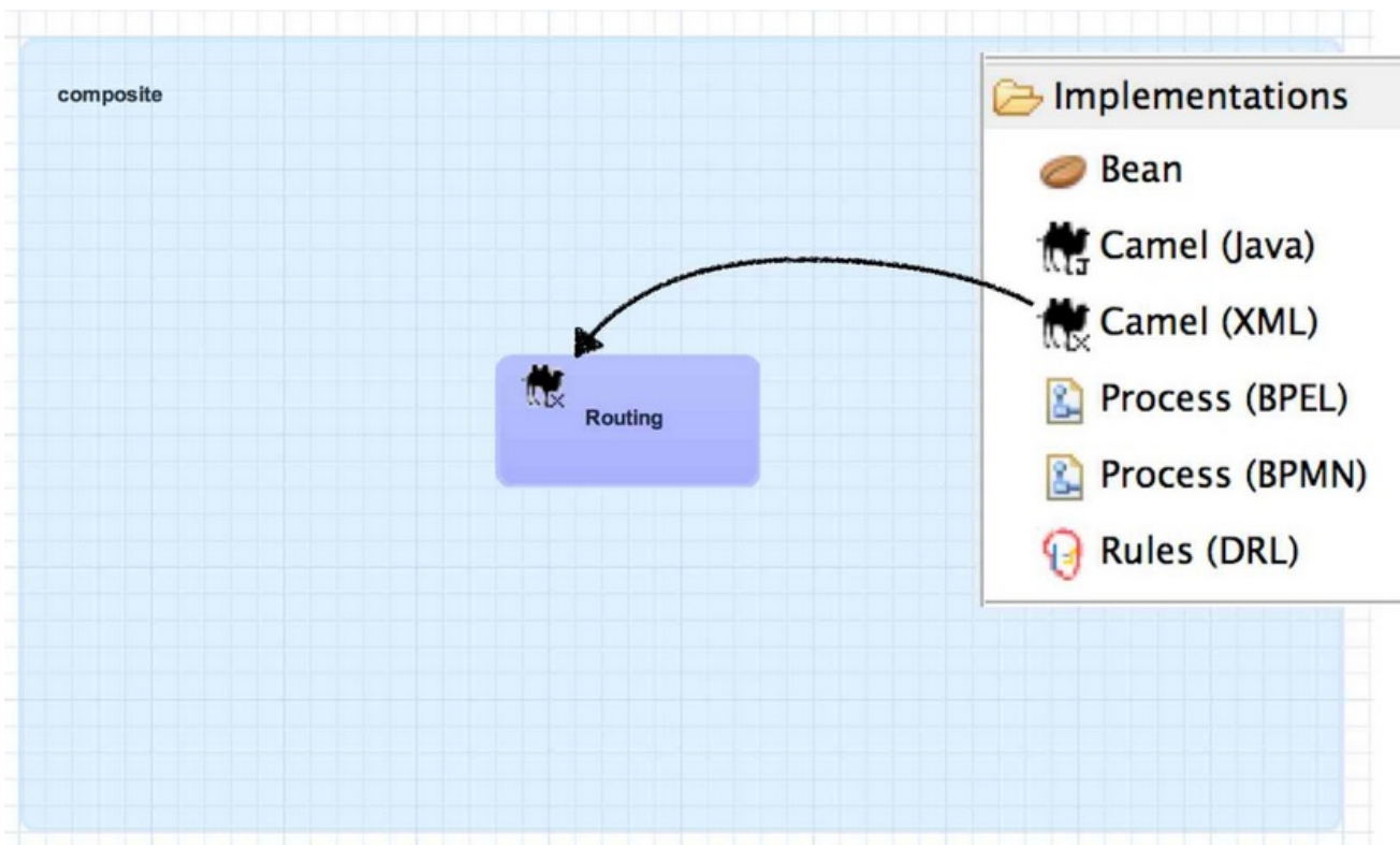
Figure 4.4. Implementation
