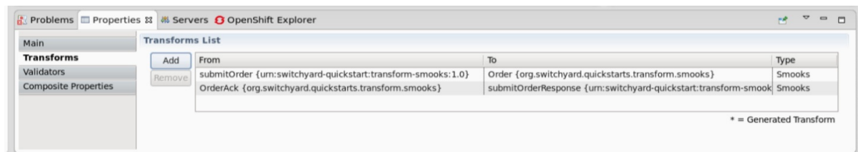
Figure 11.2. List of Transformers Under Properties View
