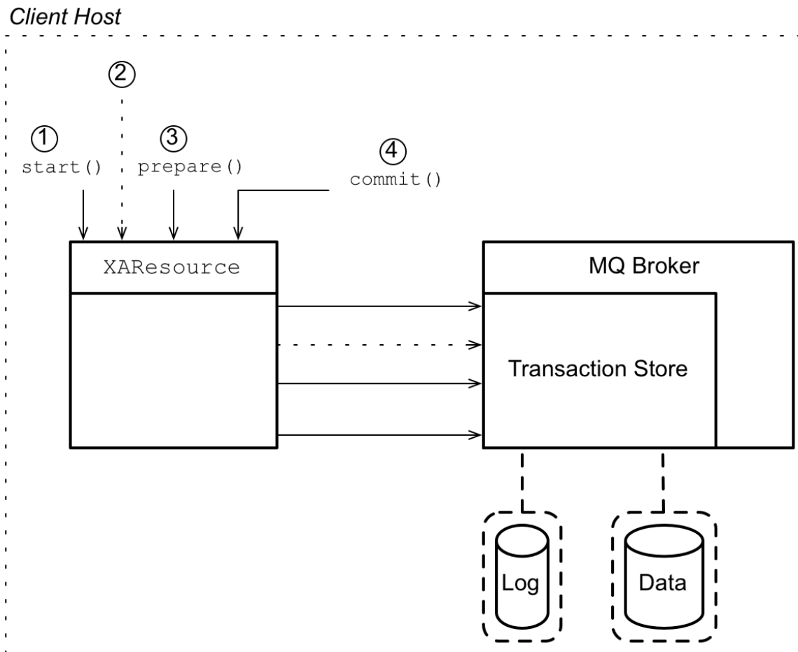
Figure 7.3. JMS XA Resource Connected to Embedded Broker
