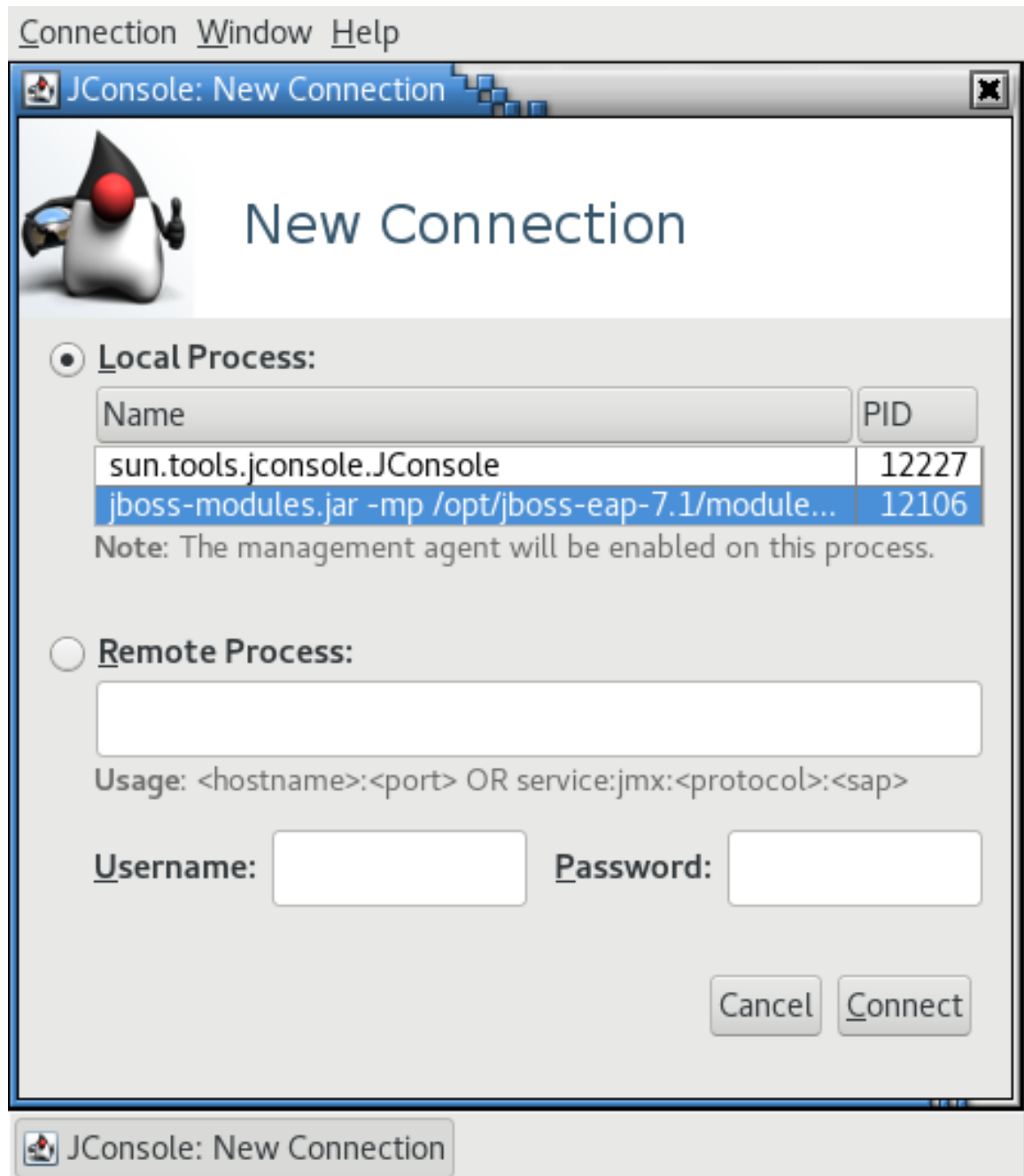
Figure 2.1. JConsole Local Standalone JBoss EAP Server JVM
