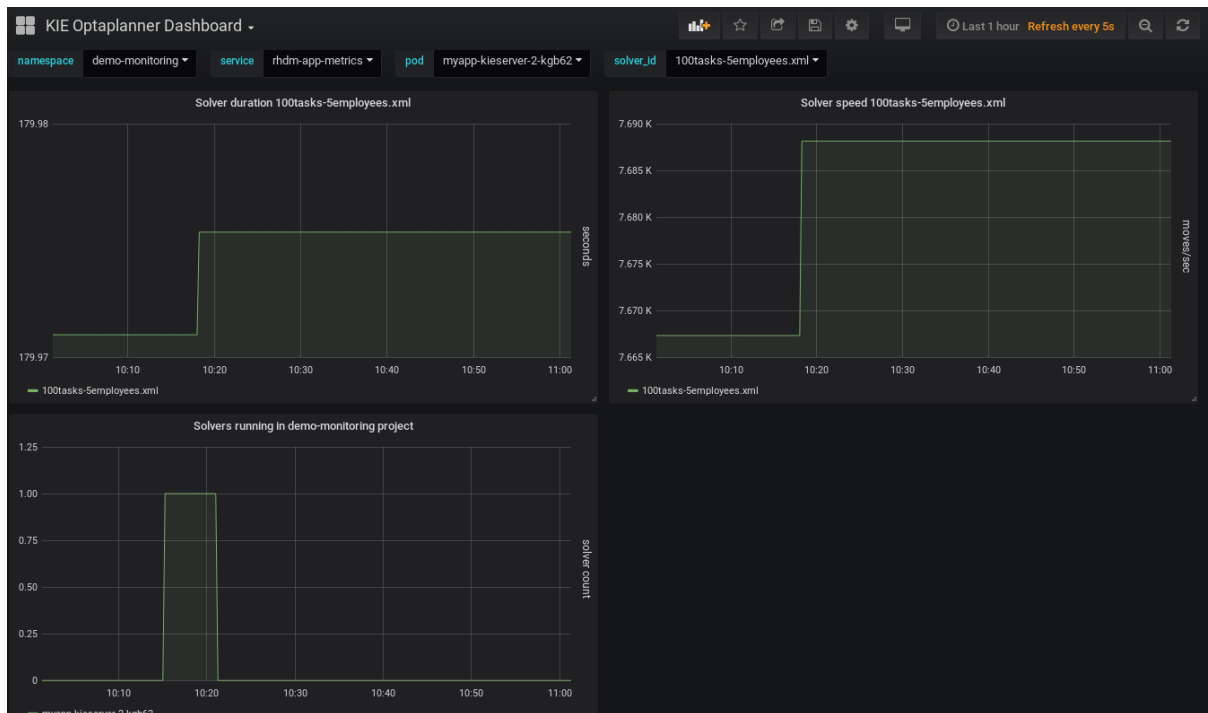
Figure 13.4. Grafana dashboard with KIE Server metrics for solvers
