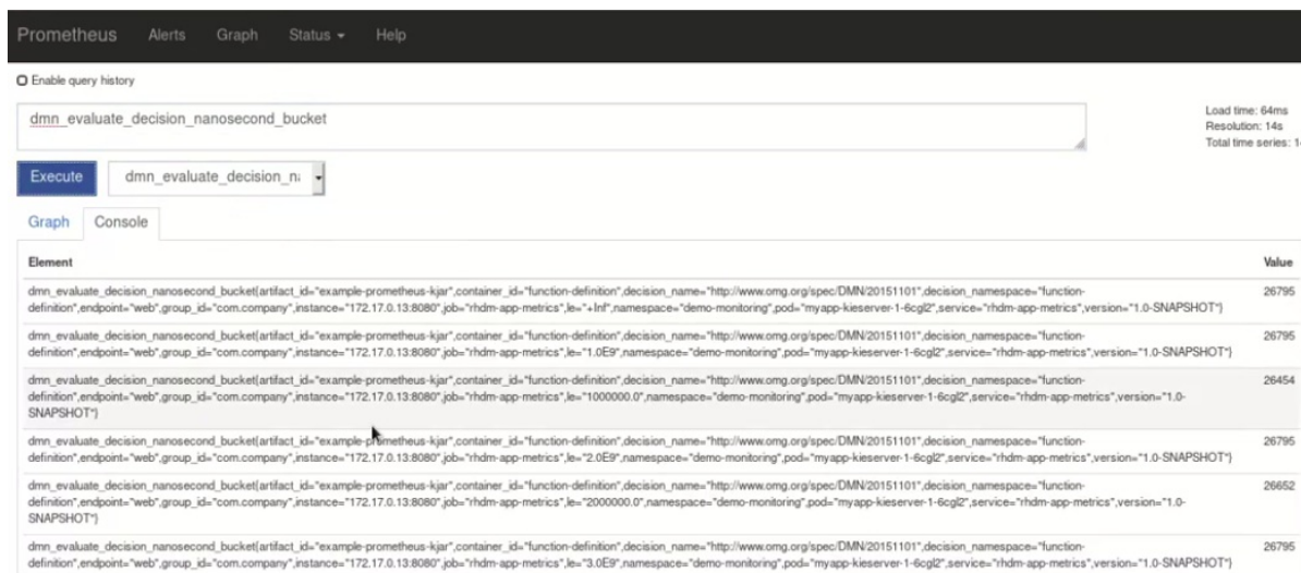
Figure 13.5. Prometheus expression browser with Decision Server metrics
