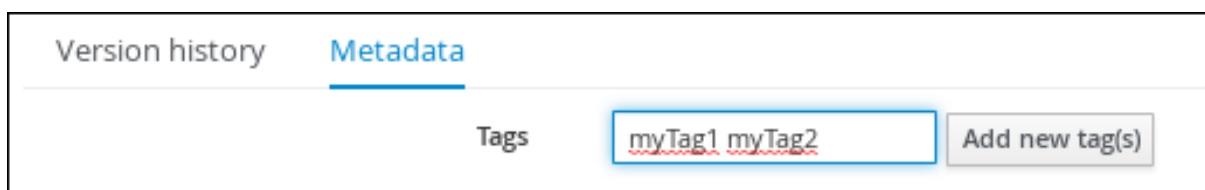
Figure 19.1. Creating tags
