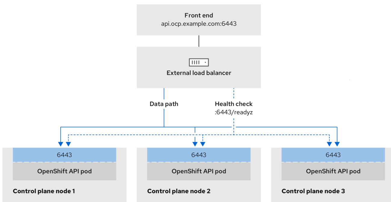
Figure 24.11. Example network workflow that shows an OpenShift API operating in an OpenShift Container Platform environment
