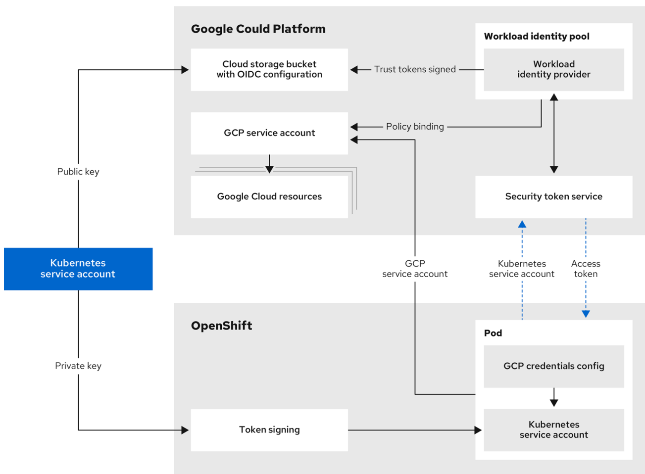
Figure 18.3. Workload Identity authentication flow
