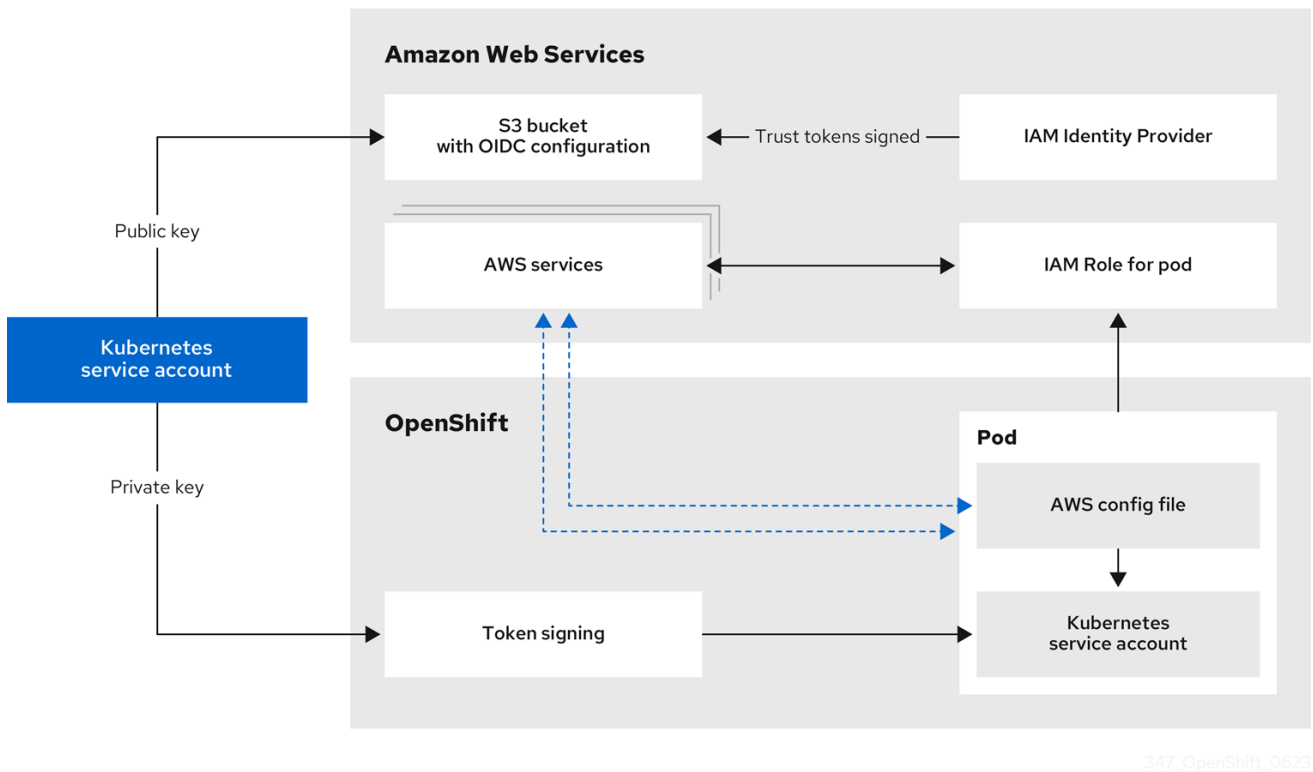
Figure 18.2. STS authentication flow
