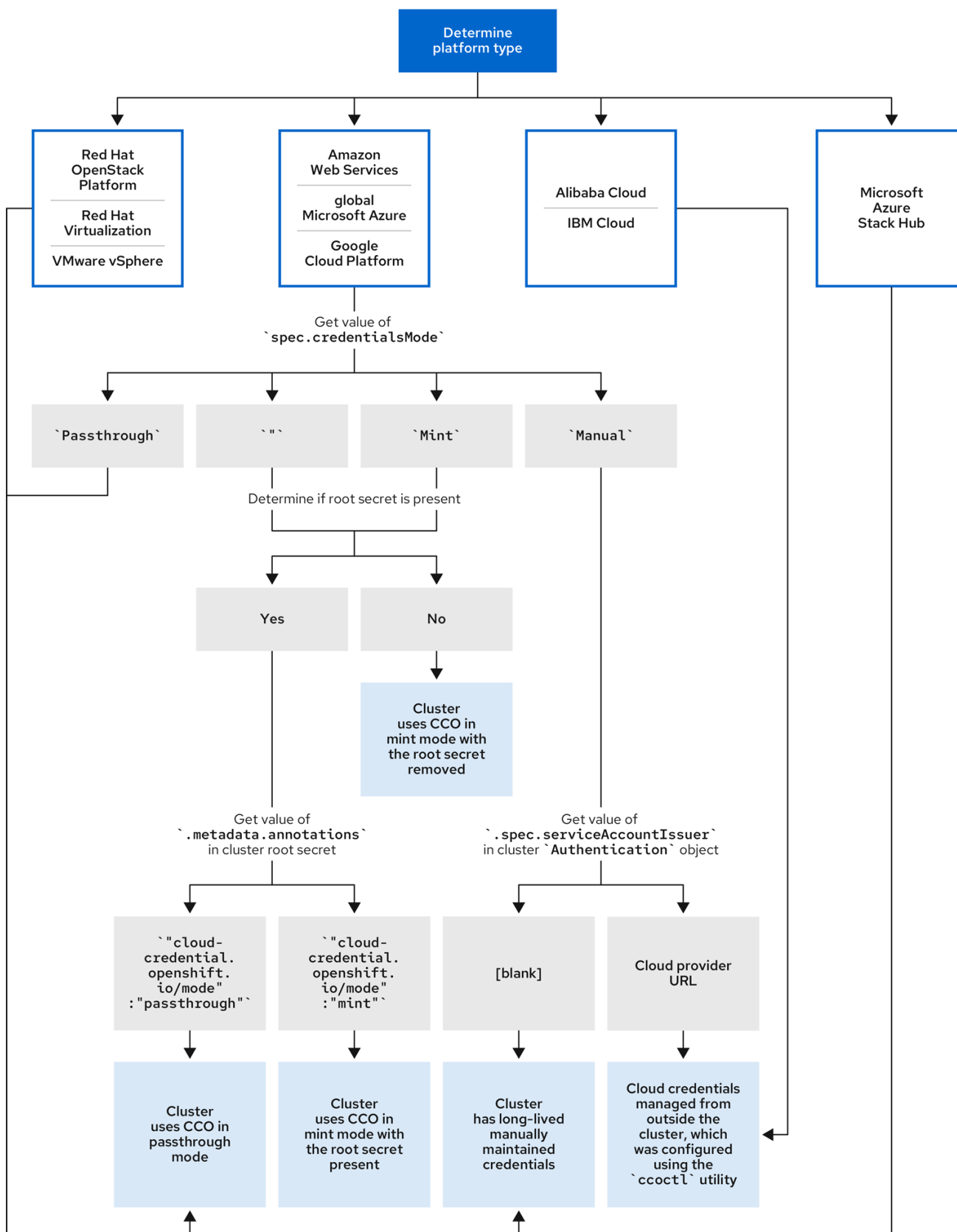
Figure 18.1. Determining the CCO configuration
