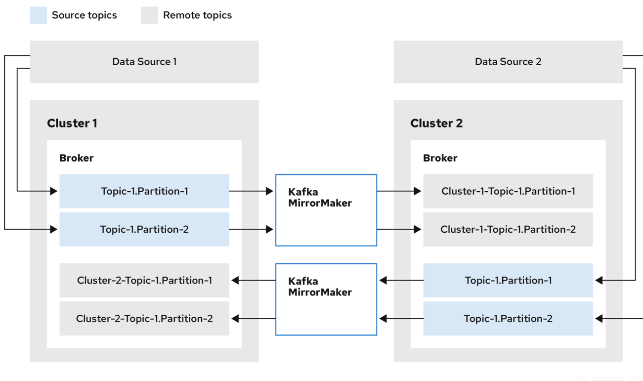
Figure 9.2. Topic renaming
