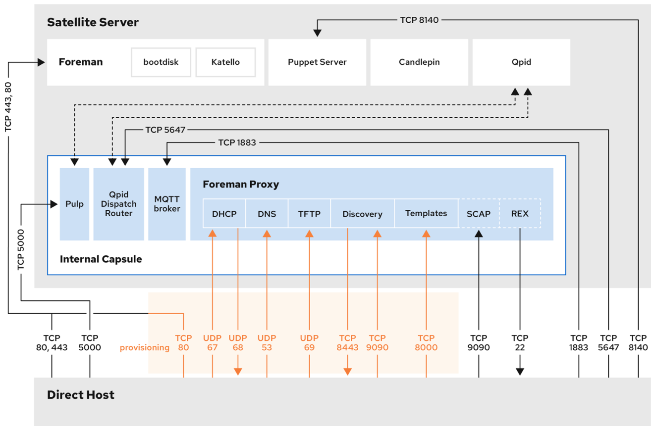
Figure 4.2. How Satellite components interact when hosts connect directly to Satellite Server
