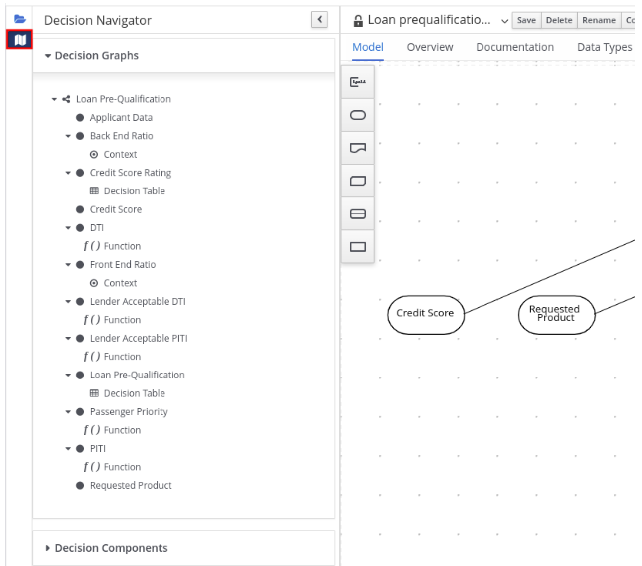
Figure 3.51. Decision Navigator view
