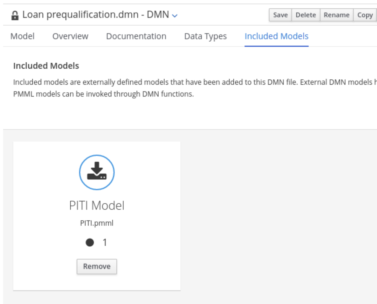
Figure 3.44. DMN file with included PMML model
