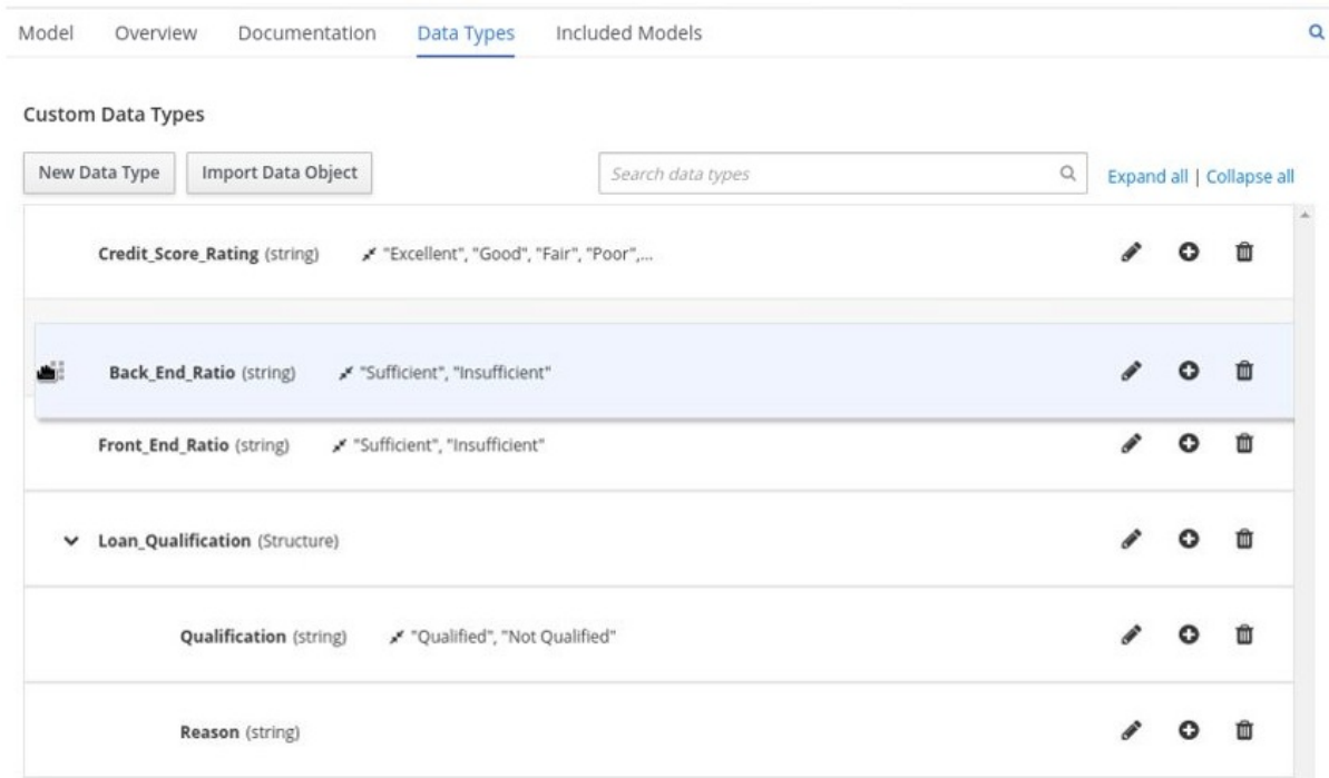
Figure 3.34. Dragging data types to change data type order or nesting
