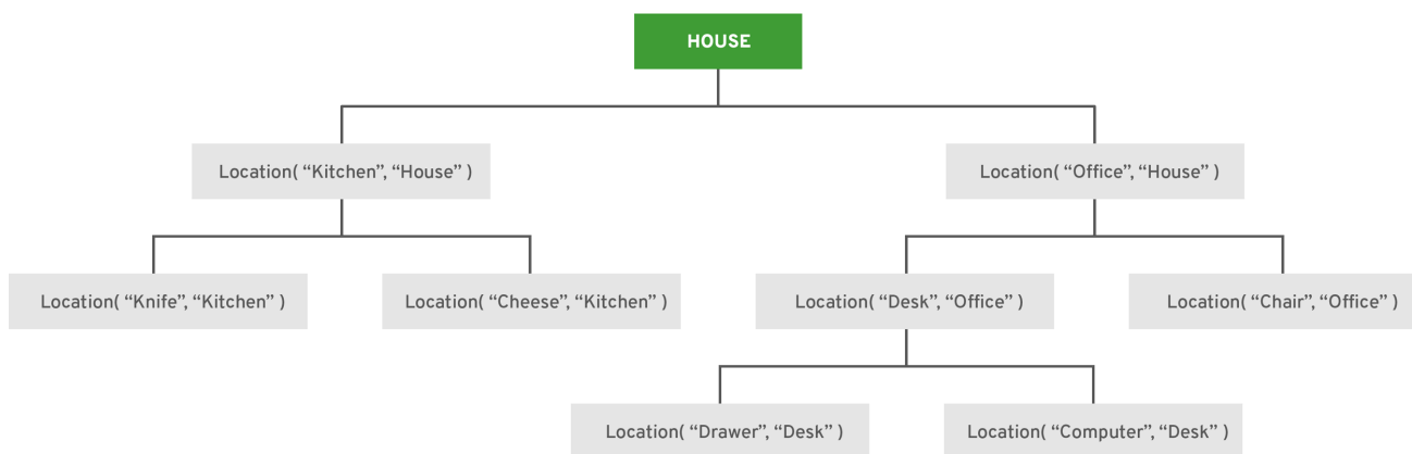
Figure 9.28. House of Doom structure
