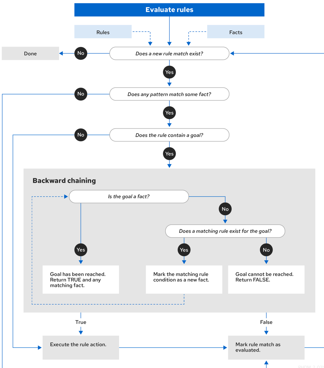
Figure 9.27. Rule evaluation logic using forward and backward chaining
