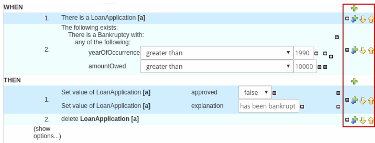
Figure 52.1. The guided rules designer
