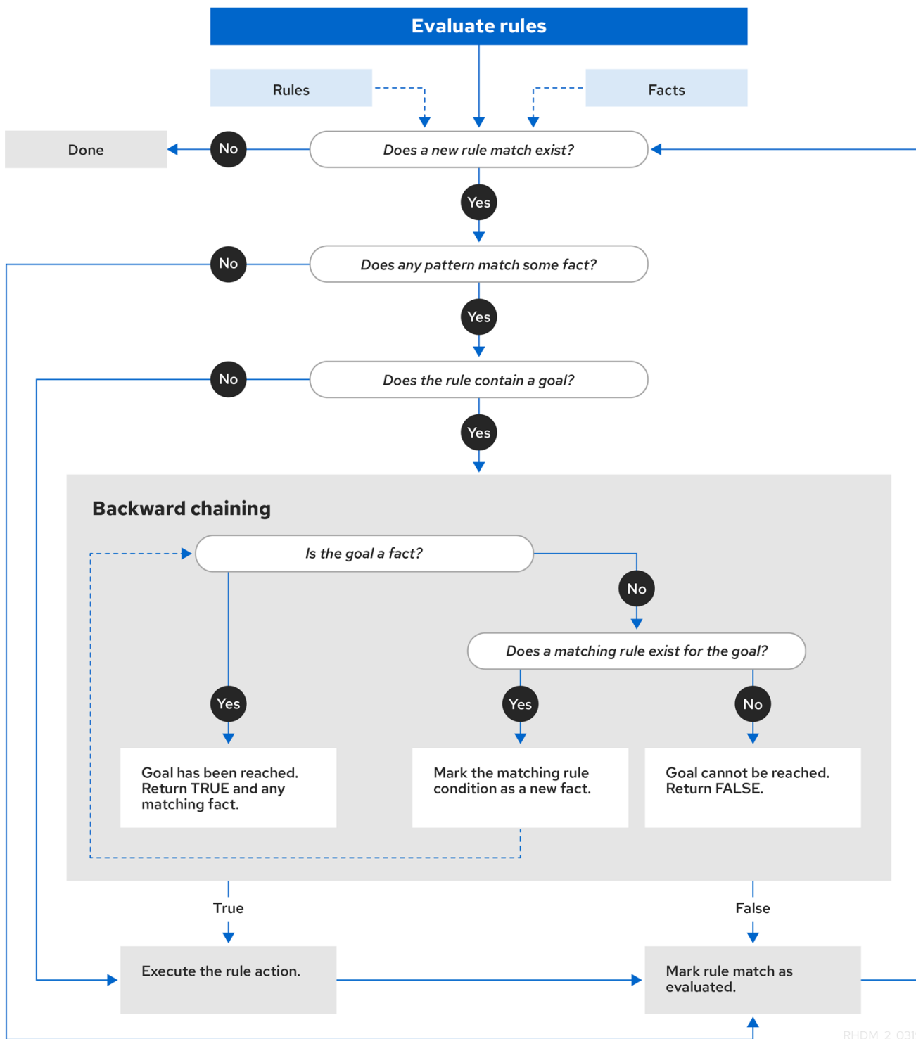
Figure 21.4. Rule evaluation logic using forward and backward chaining
