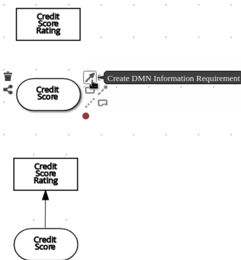
Figure 6.8. Connecting credit score input to the credit score rating decision
