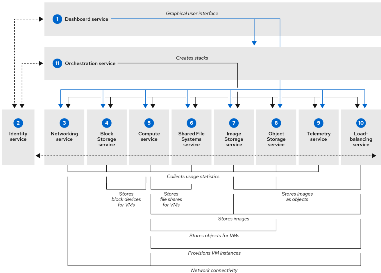
Figure 2.1. RHOSP core services and their relationships
