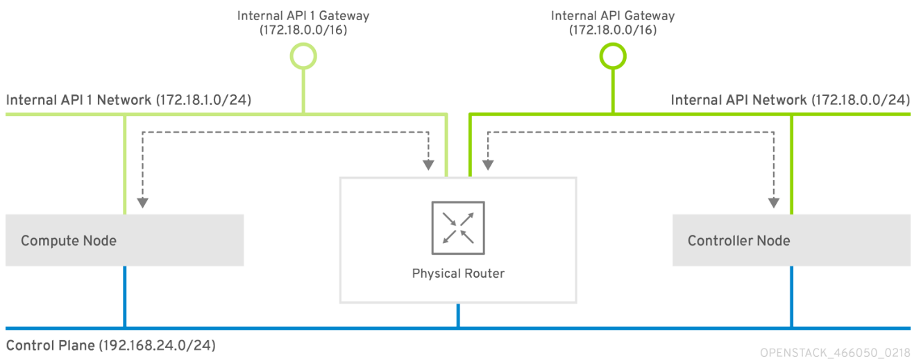
Figure 4.2. Routed traffic through Internal API
