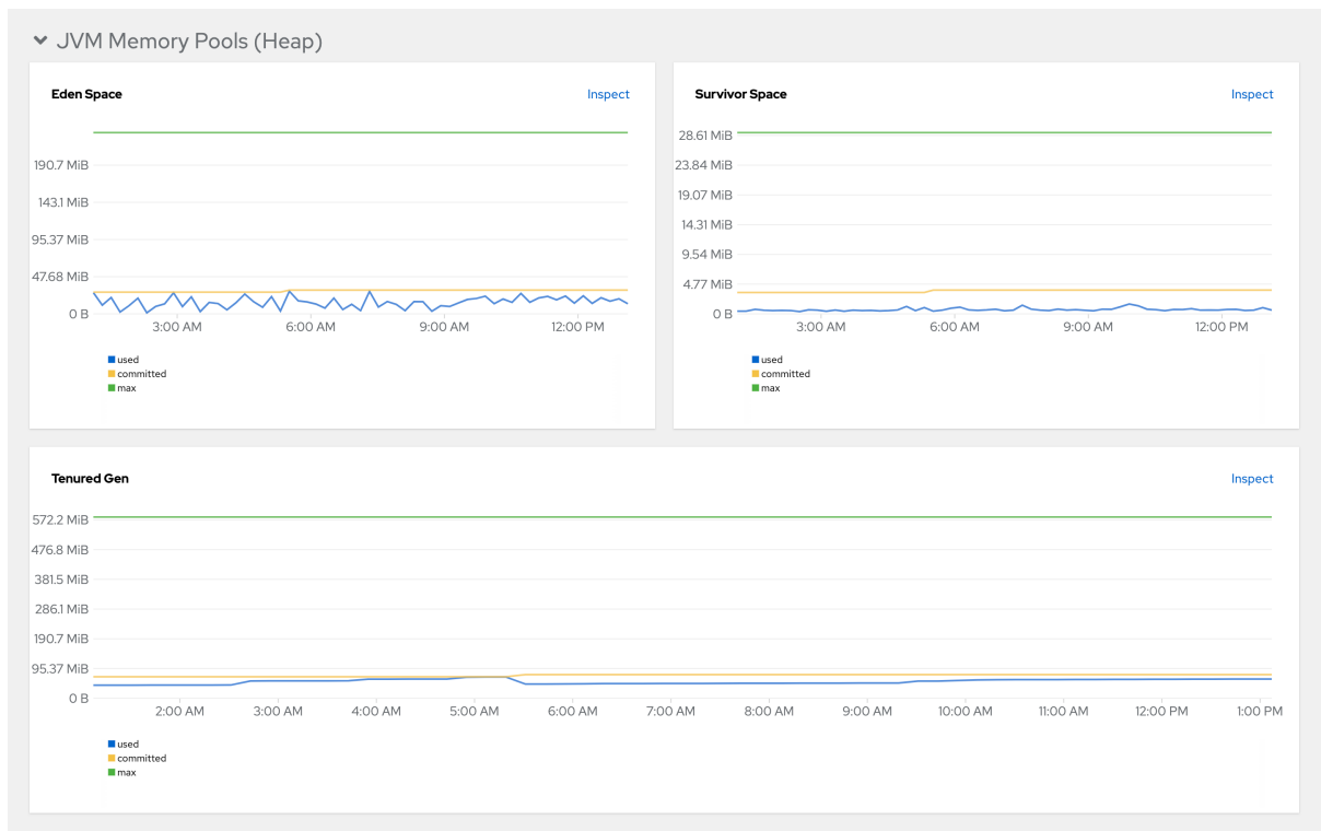
Figure 3.6. JVM Memory Pools (heap)
