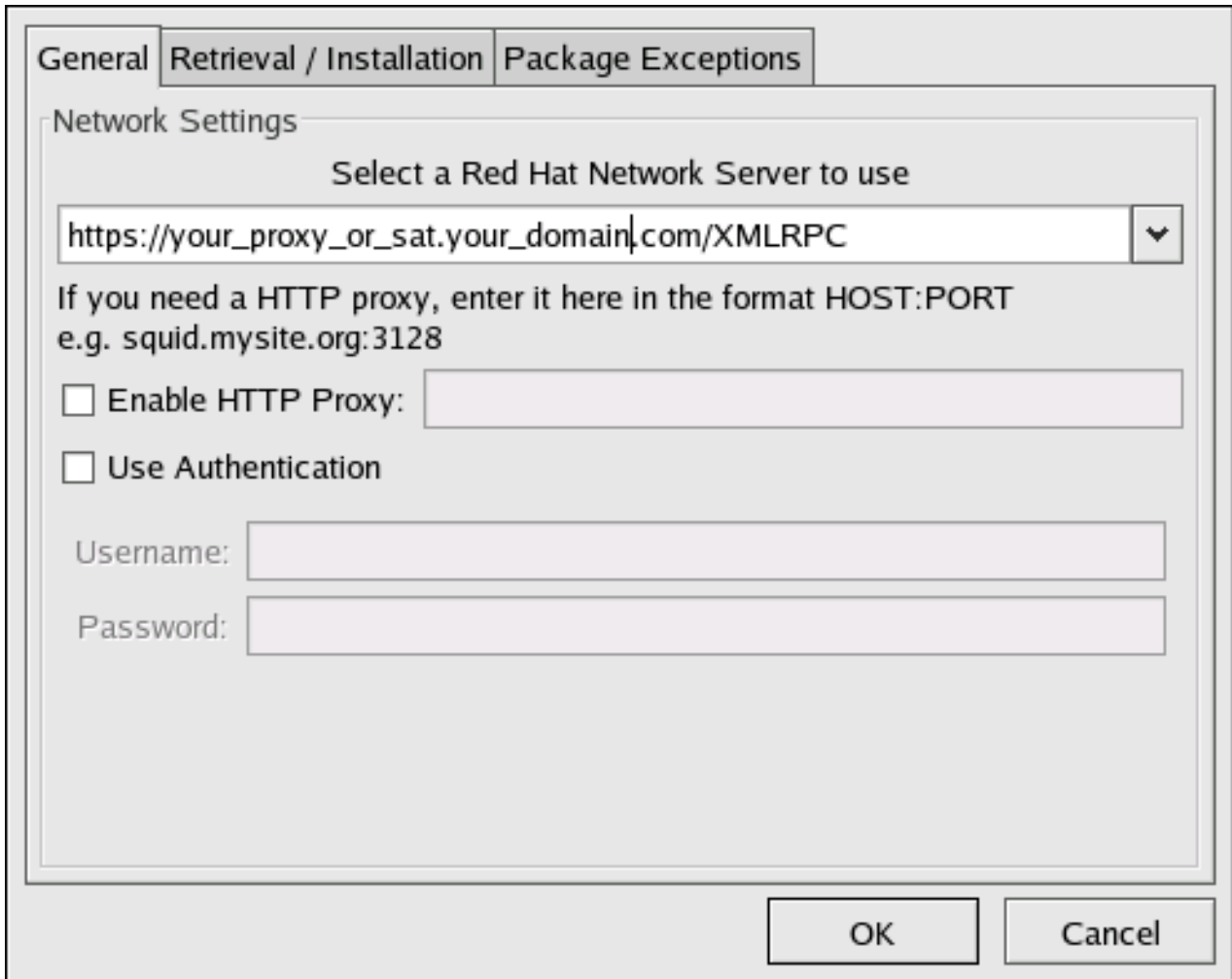
Figure 2.1. Red Hat Update Agent GUI Configuration
