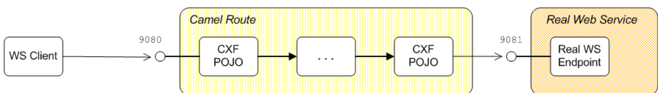
Figure 41.2. Proxy Route with Message in POJO Format
