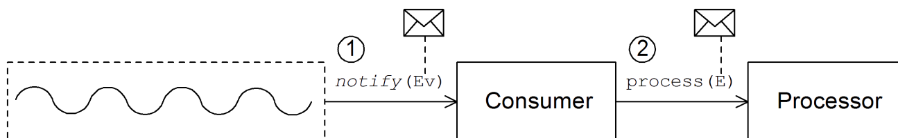
Figure 47.3. Event-Driven Consumer
