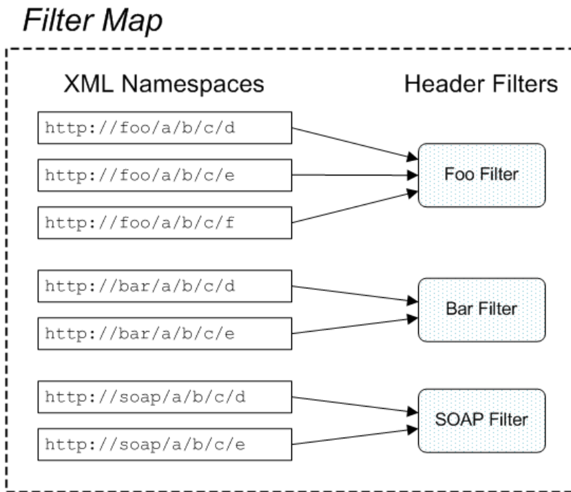
Figure 42.1. Filter Map
