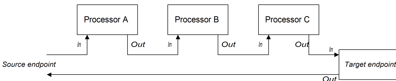
Figure 44.1. Pipelining Model
