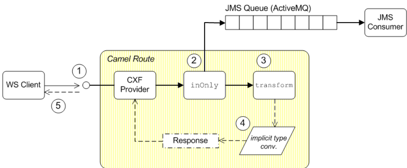
Figure 40.2. SOAP/HTTP-to-JMS Bridge
