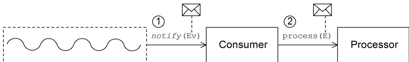
Figure 38.3. Event-Driven Consumer
