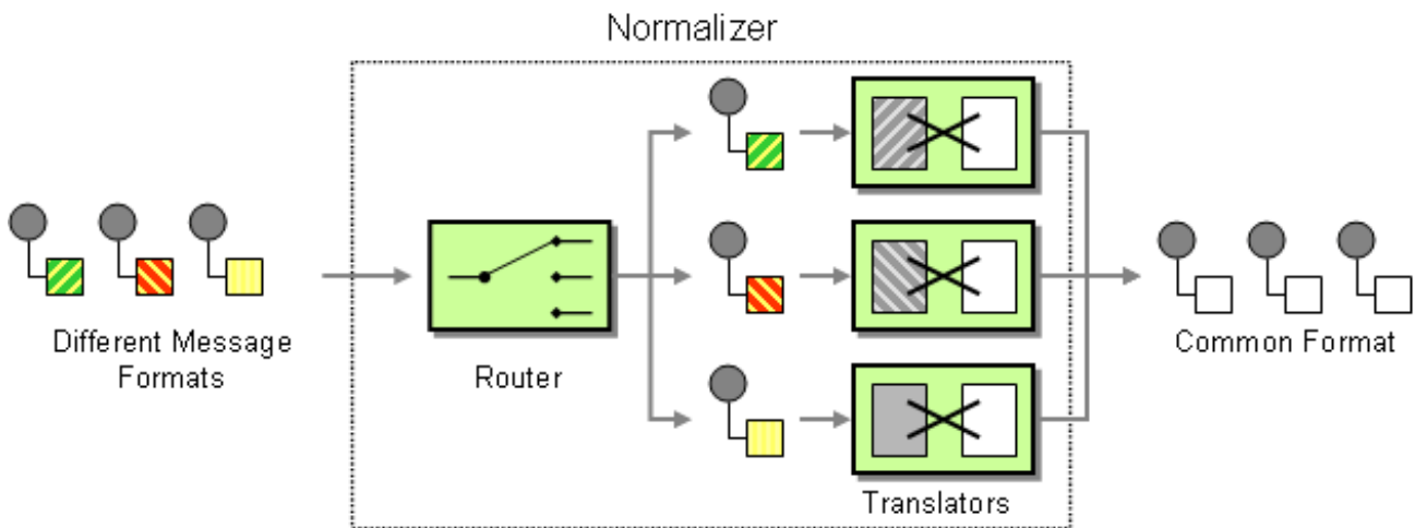
Figure 10.3. Normalizer Pattern
