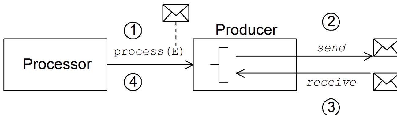
Figure 38.6. Synchronous Producer
