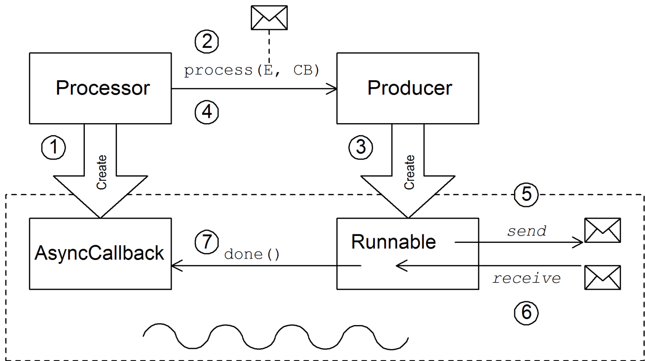
Figure 38.7. Asynchronous Producer
