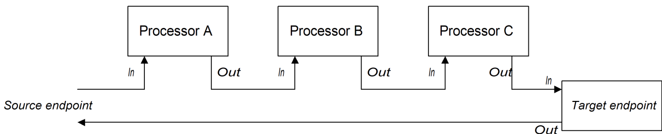
Figure 35.1. Pipelining Model
