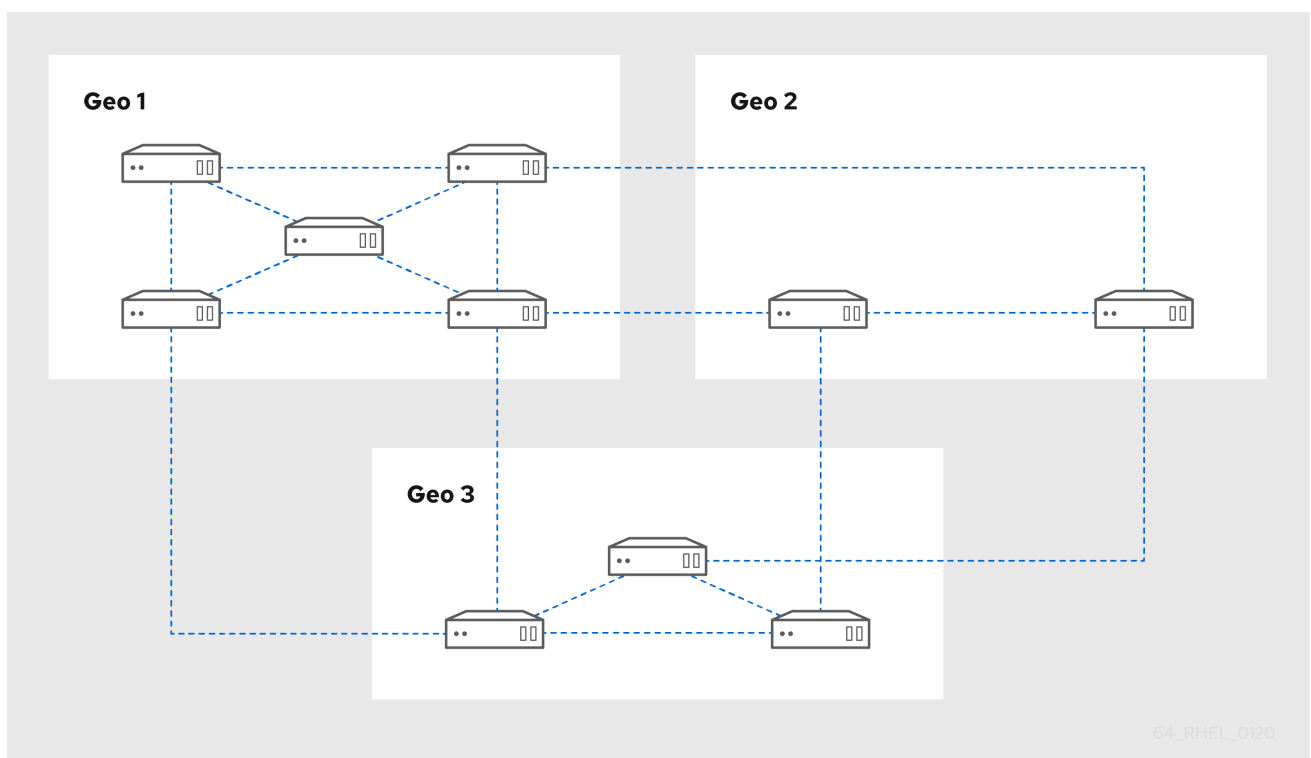
Figure 3.3. Replica Topology Example 2
