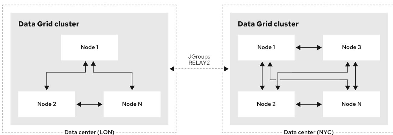
Figure 1.1. Cross-site replication
