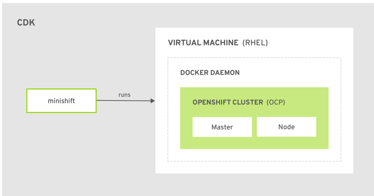
Figure 2.1 : CDK architecture
