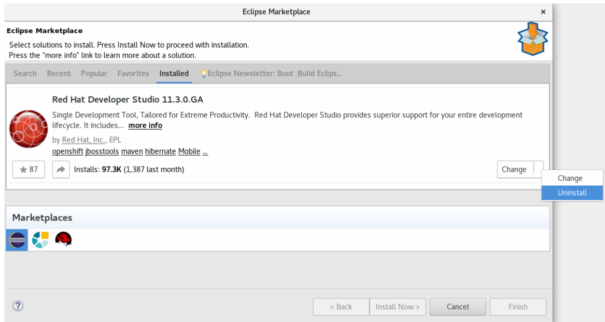
Figure 4.2. Uninstall Button
