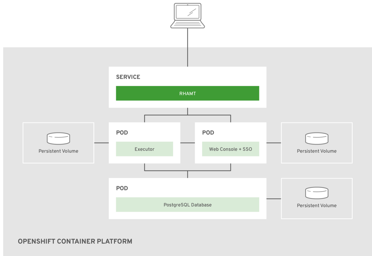
Figure 2.2. web-template.json
