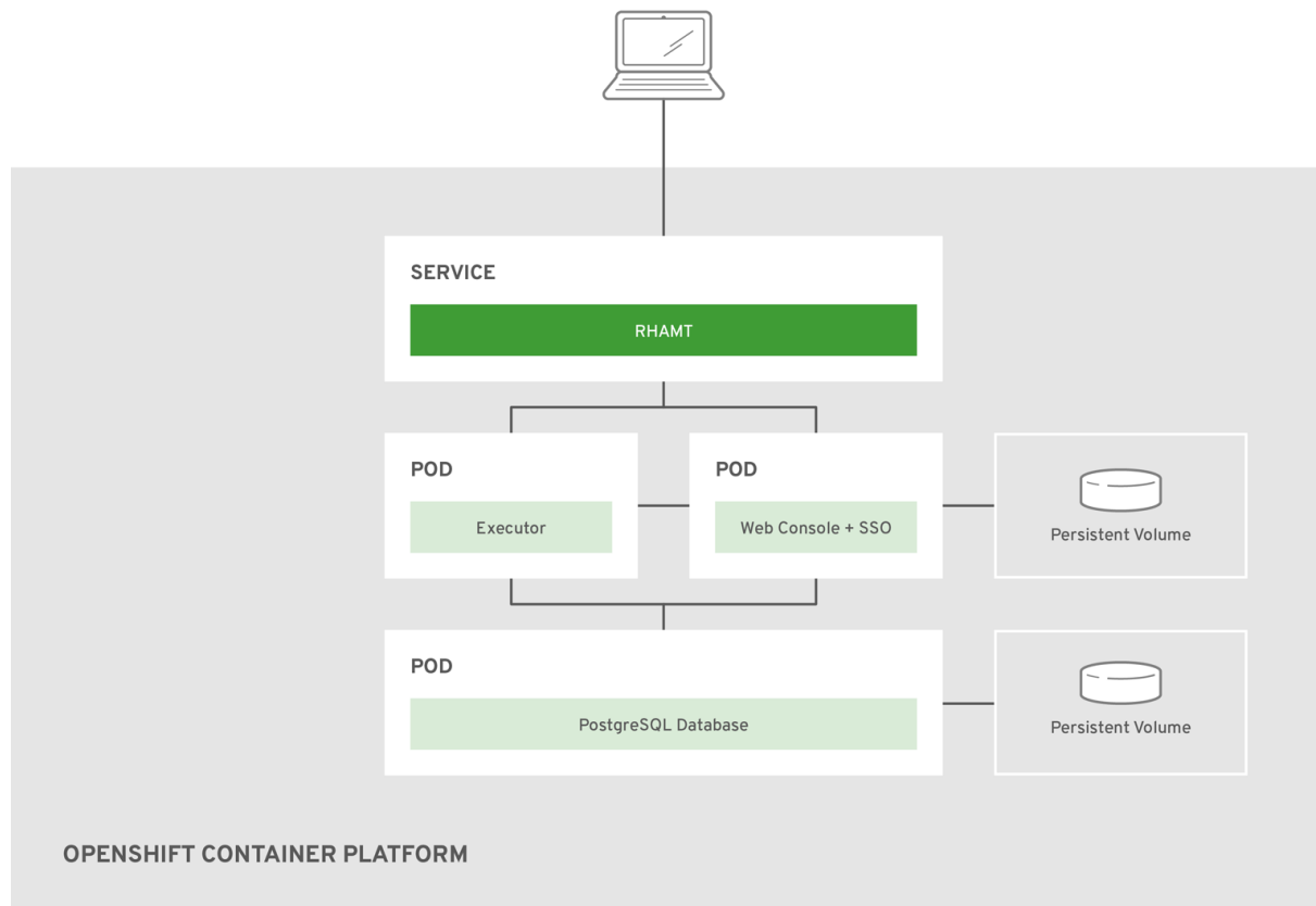
Figure 2.3. web-template-empty-dir-executor.json
