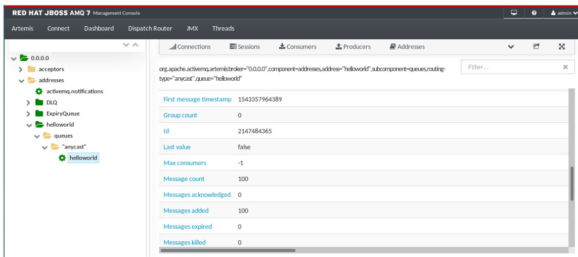
Figure 4.1. Message count
