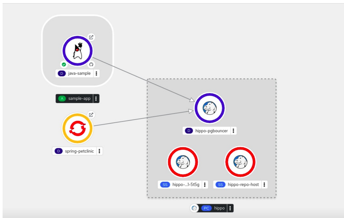
Figure 5.2. Connecting multiple applications
