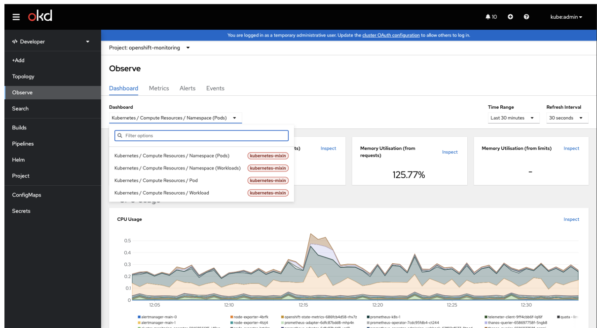
Figure 10.1. Observe dashboard
