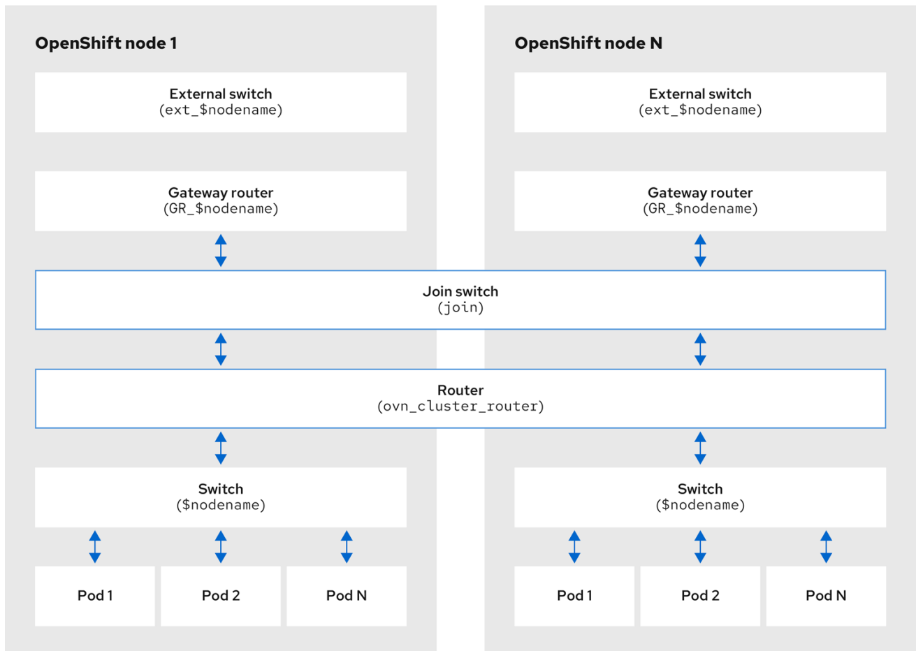
Figure 27.2. OVN-Kubernetes router and switch components
