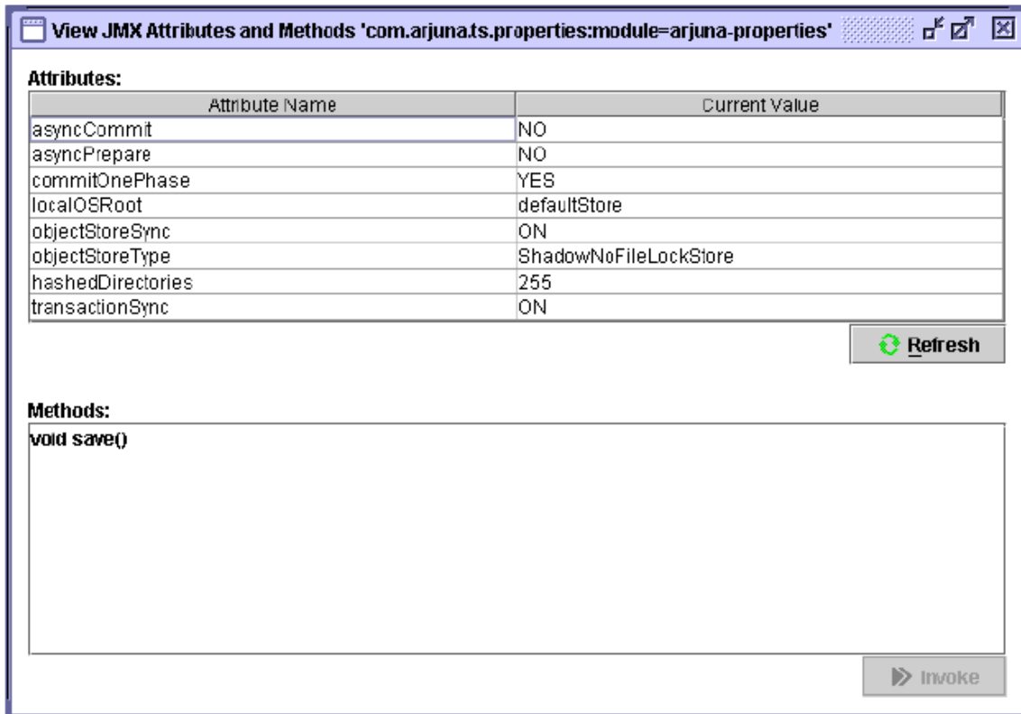
View JMX Attributes and Operations window
