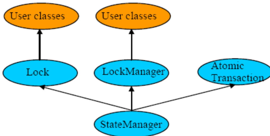
Figure 1: Txcore class hierarchy
