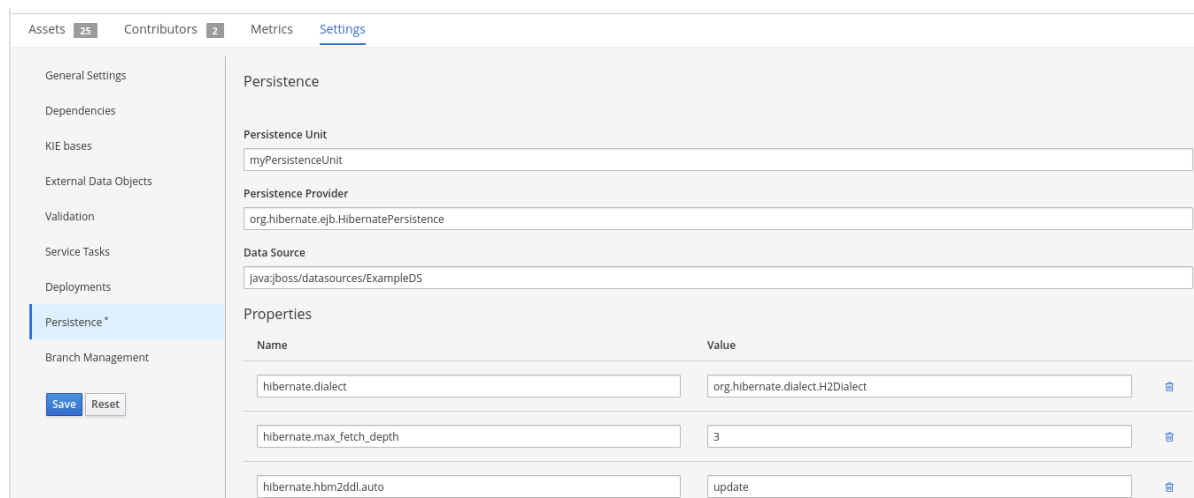
Figure 20.3. Persistence unit and data source configuration in Business Central
