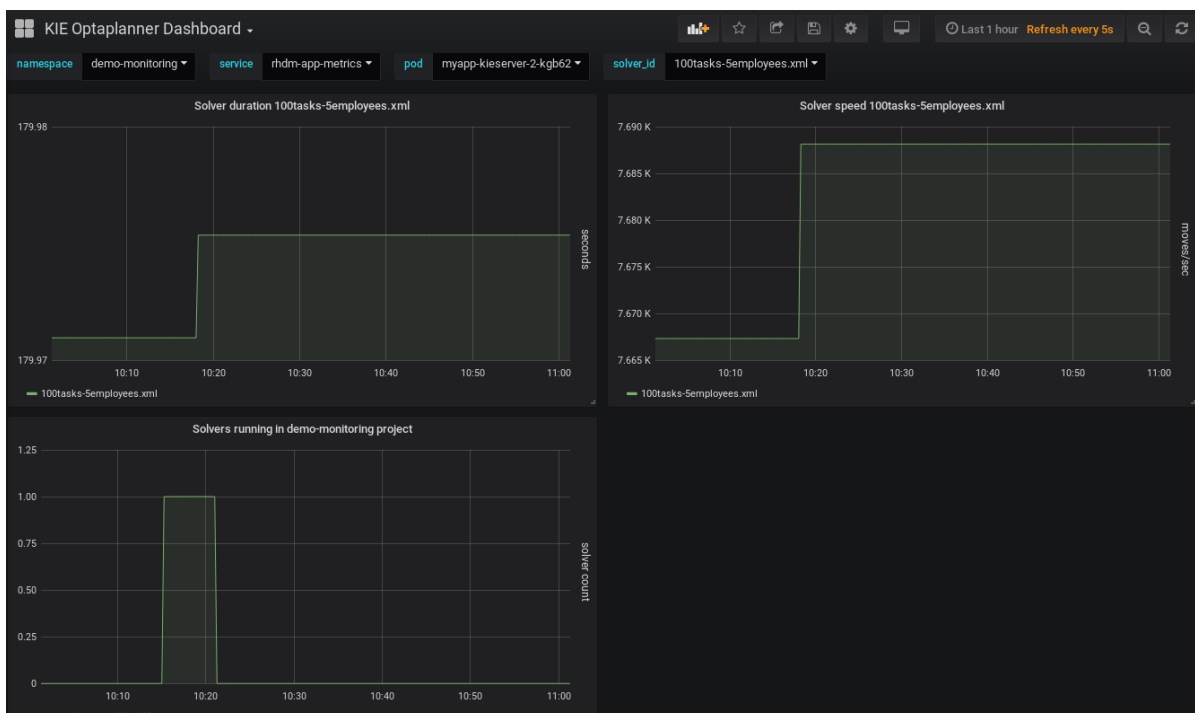
Figure 18.4. Grafana dashboard with KIE Server metrics for solvers
