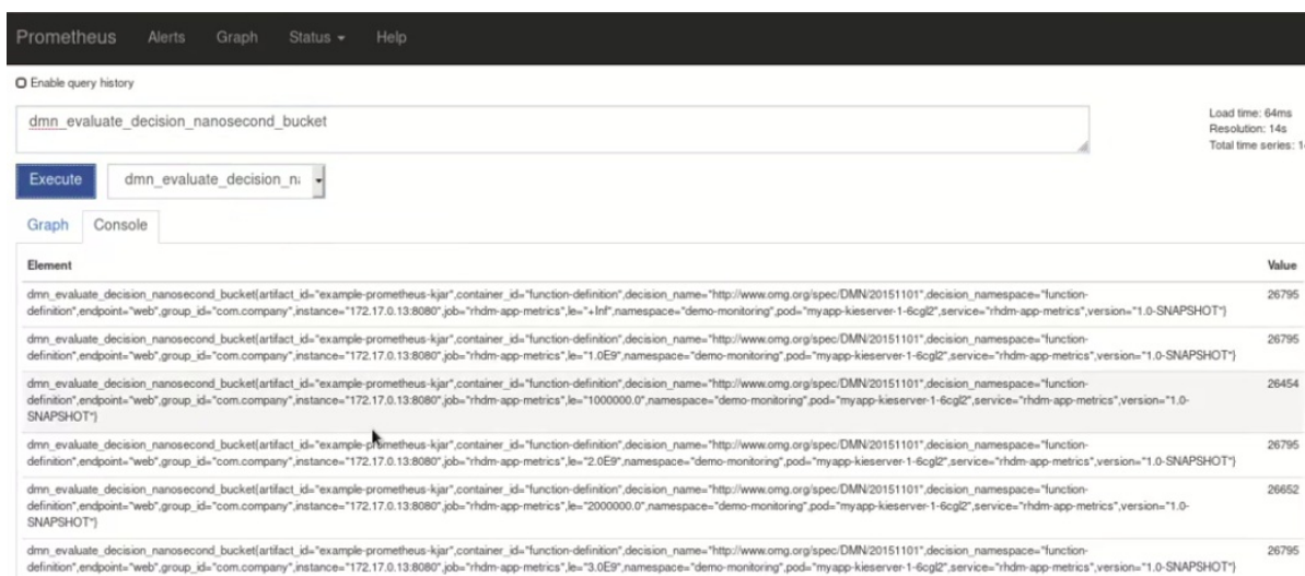
Figure 18.1. Prometheus expression browser with KIE Server metrics
