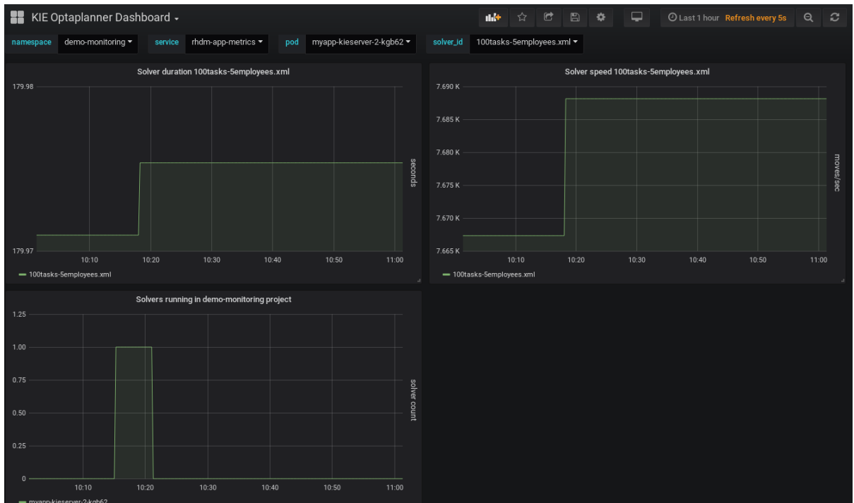
Figure 18.9. Grafana dashboard with KIE Server metrics for solvers
