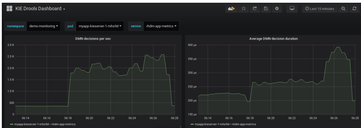
Figure 18.3. Grafana dashboard with KIE Server metrics for DMN models
