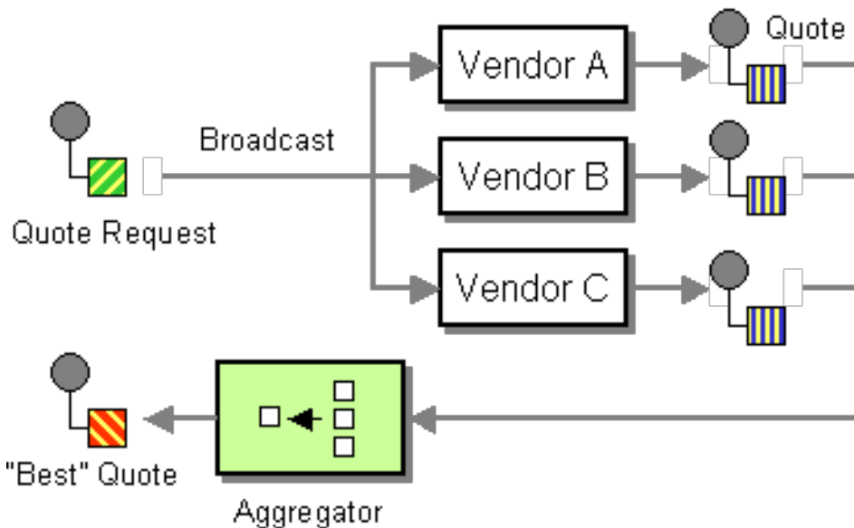
Figure 8.11. Scatter-Gather Pattern
