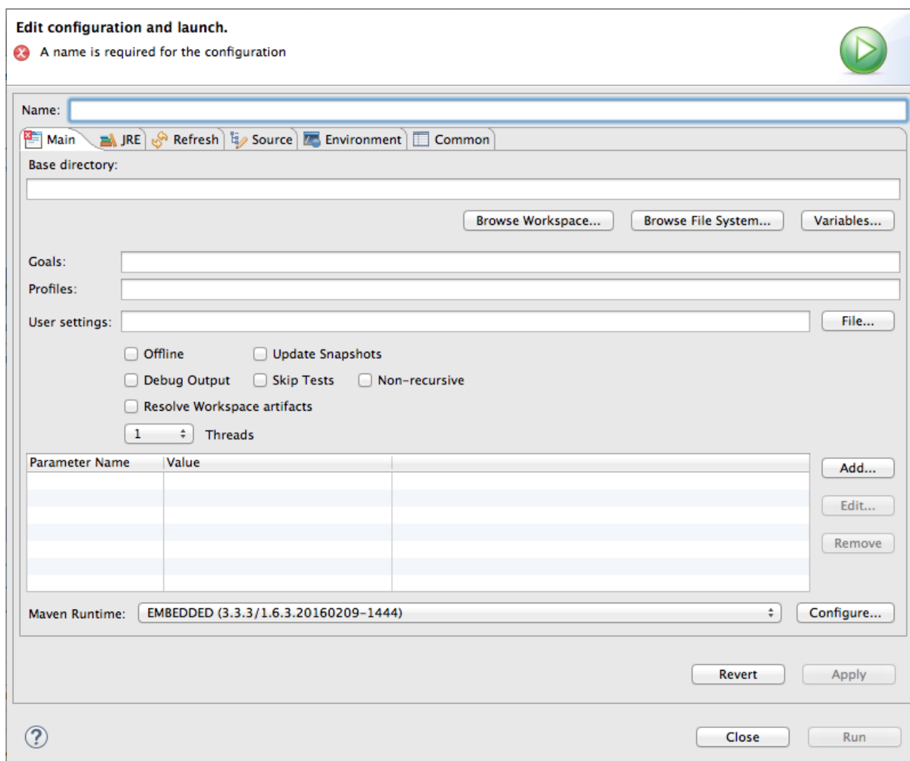
Figure 6.2. Runtime configuration editor for Maven
