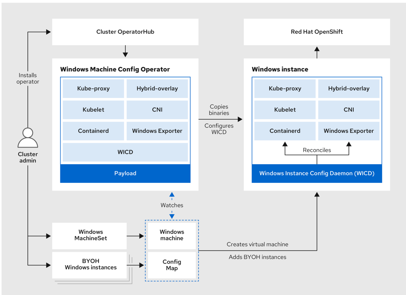
Figure 4.1. WMCO design
