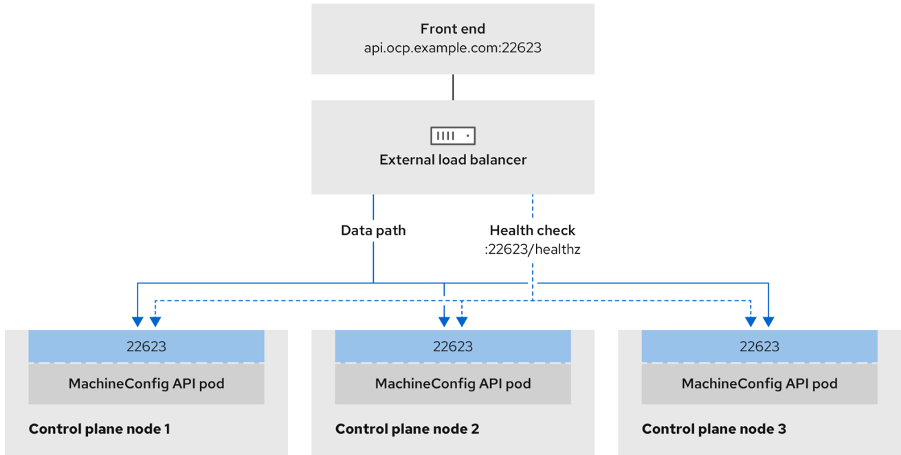
Figure 32.3. Example network workflow that shows an OpenShift MachineConfig API operating in an OpenShift Container Platform environment
