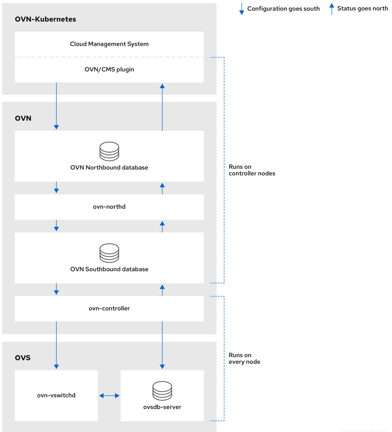
Figure 25.1. OVK-Kubernetes architecture
