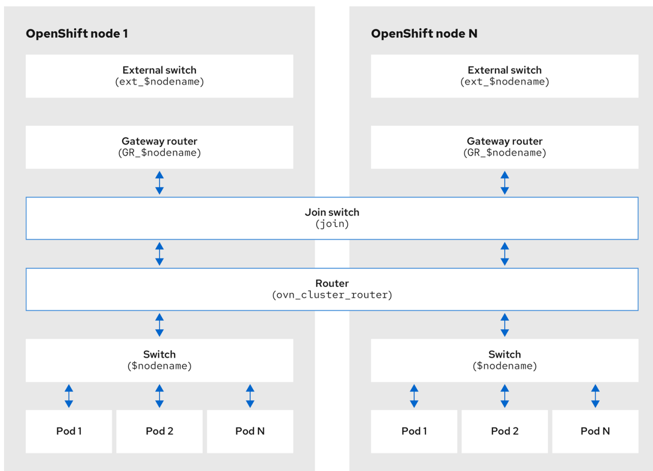
Figure 25.2. OVN-Kubernetes router and switch components
