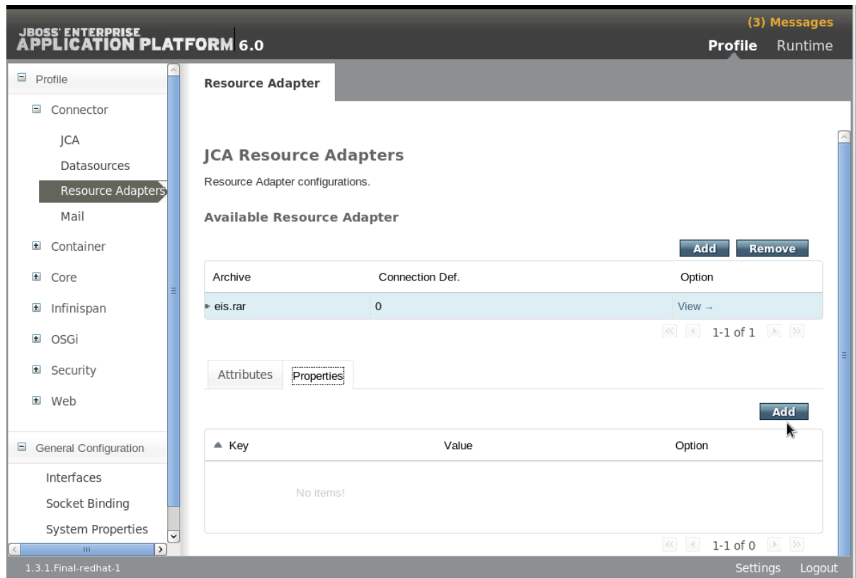
Figure 17.12. Add Resource Adapter Properties
