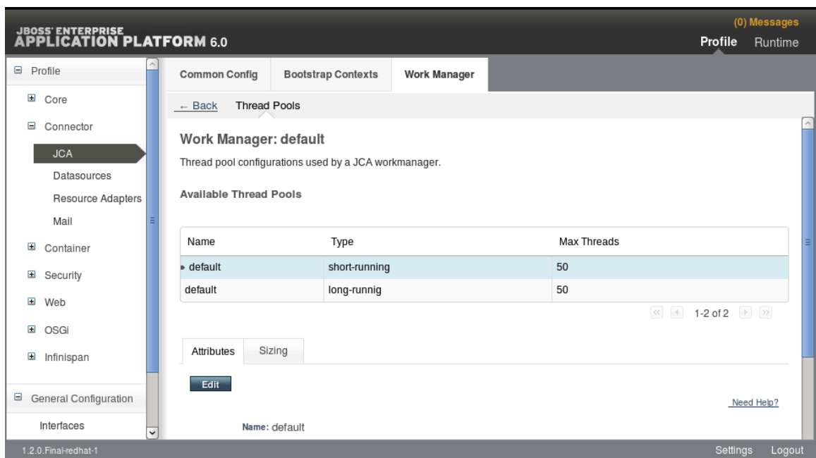
Figure 17.3. Work Manager Thread Pools
