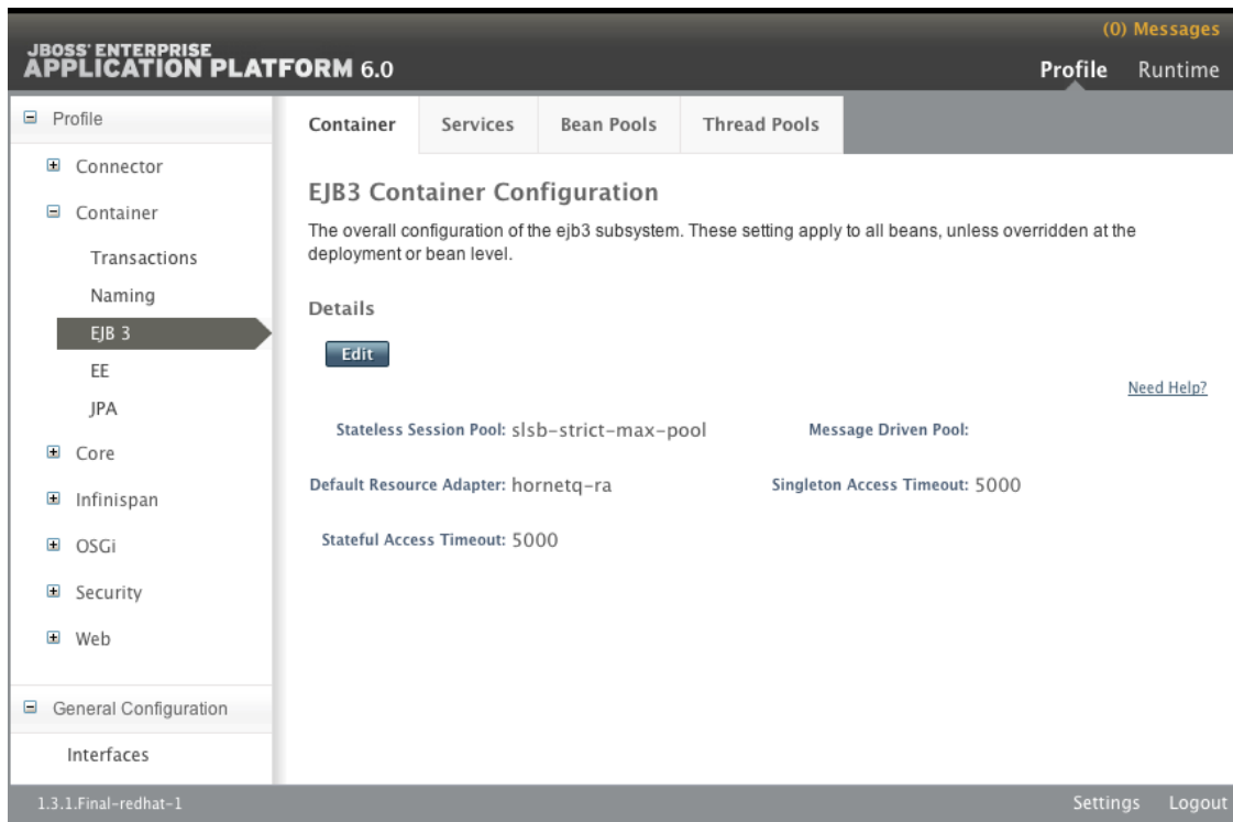
Figure 16.1. EJB Configuration Options in the Management Console (Standalone Server)
