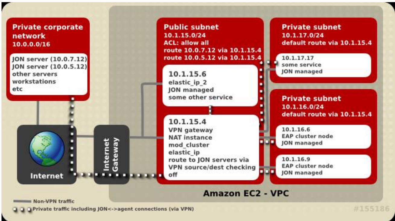
Figure 18.1. JON Server connectivity
