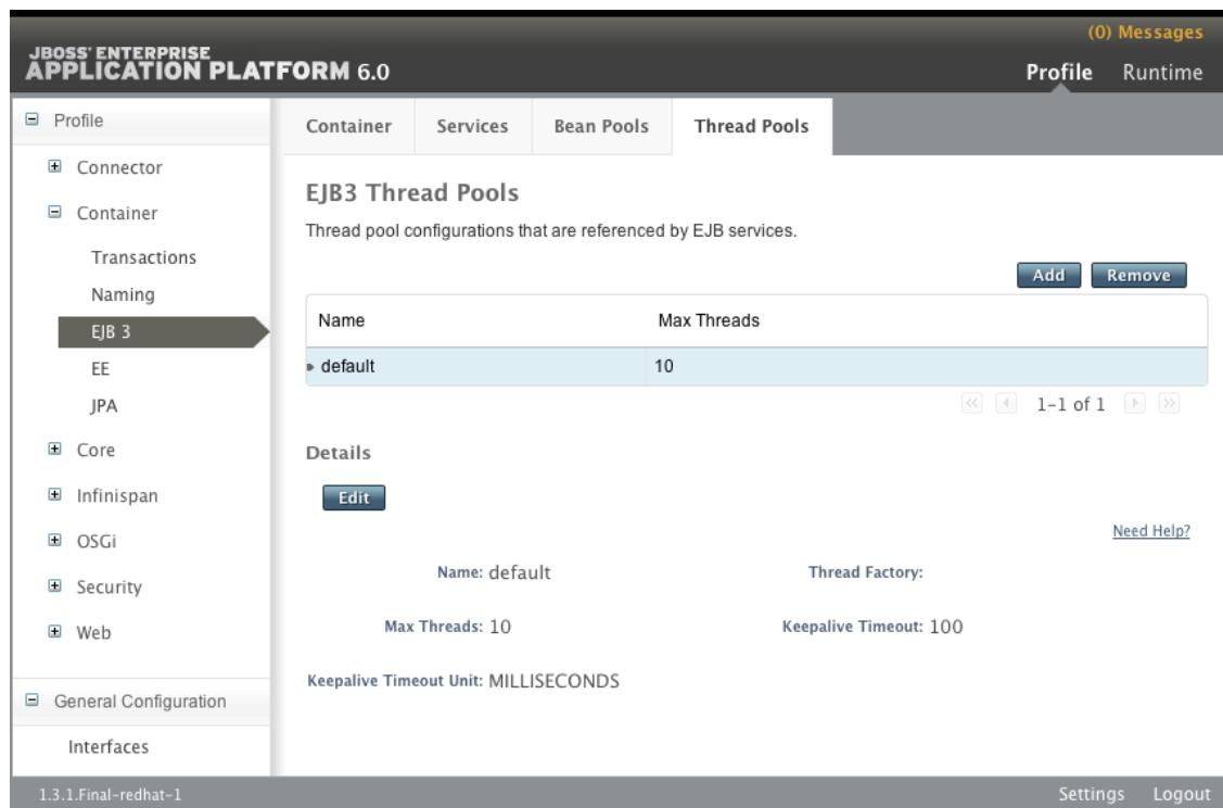
Figure 16.6. EJB3 Thread Pools Panel
