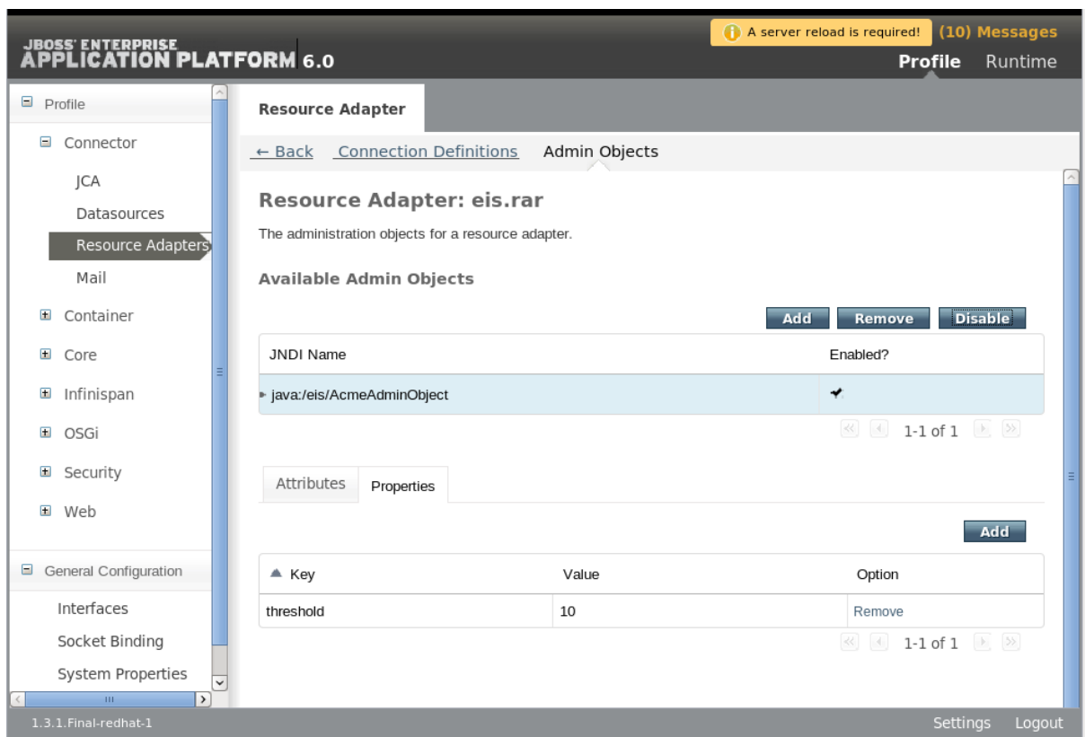
Figure 17.27. Connection Definition Enabled
