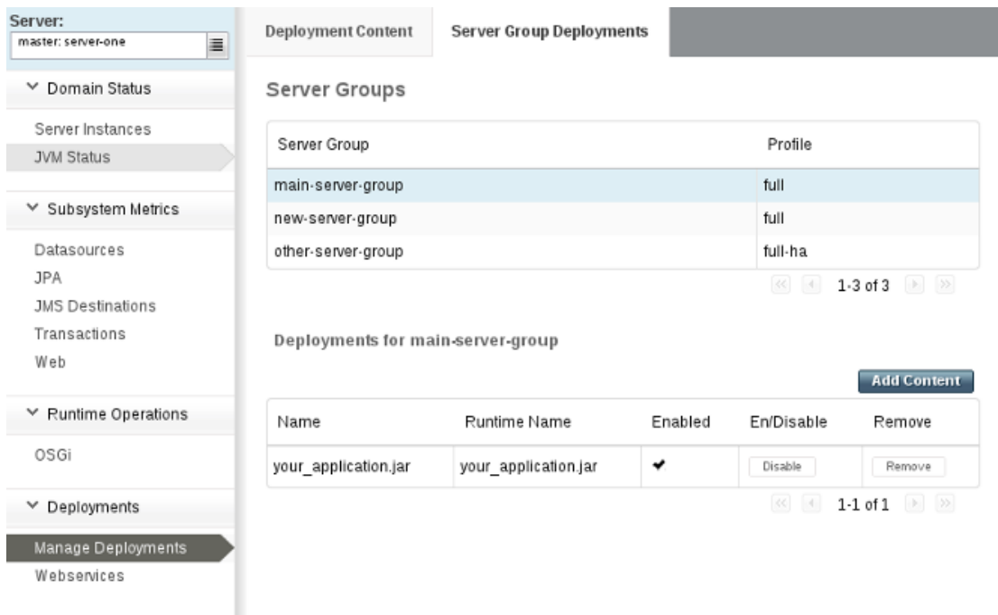
Figure 8.5. Confirmation of application deployment to server groups
