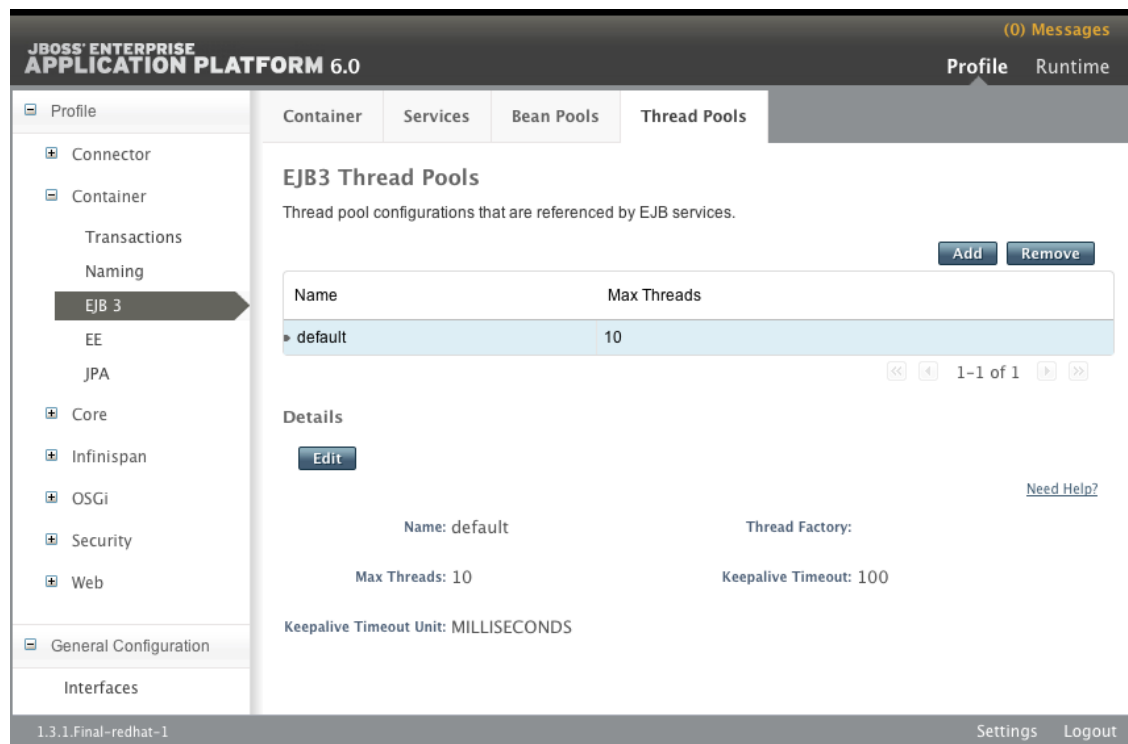
Figure 16.8. EJB3 Thread Pools Tab
