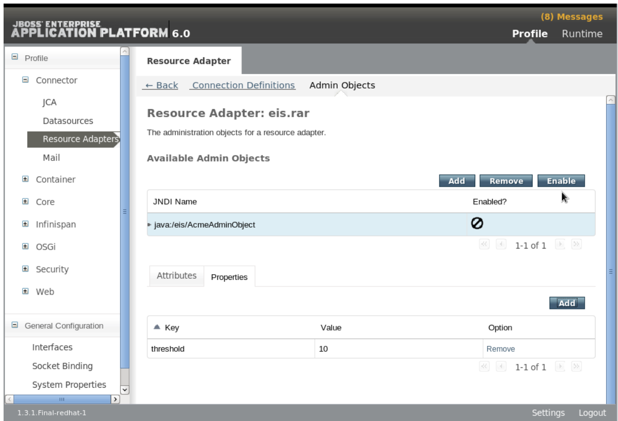
Figure 17.26. Admin Object - Disabled
