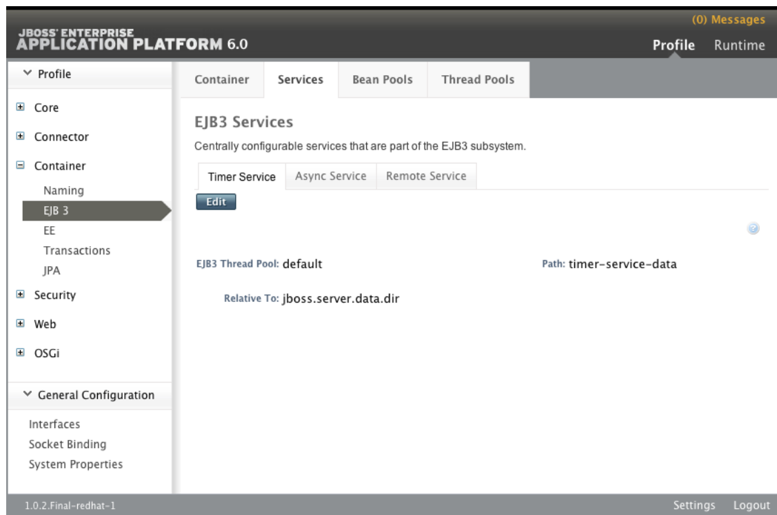
Figure 16.11. Timer Service tab of the EJB3 Services panel
