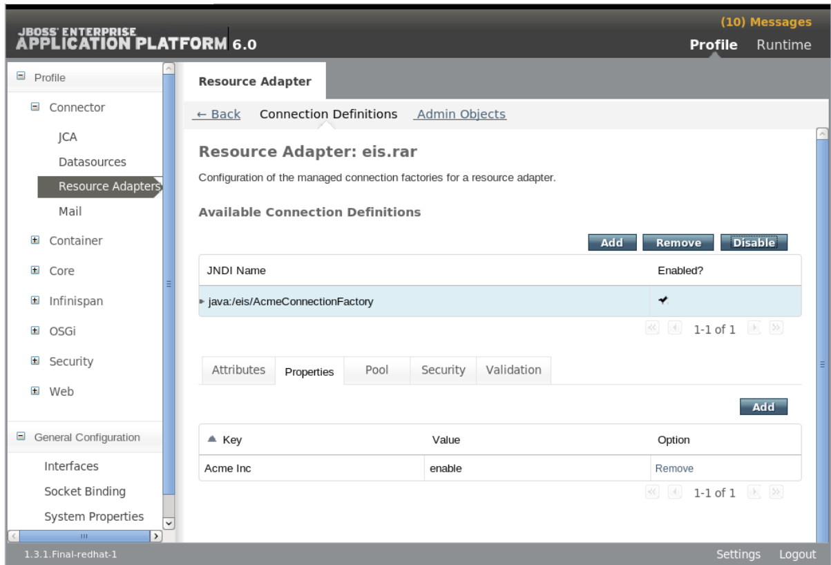
Figure 17.21. Connection Definition Enabled
