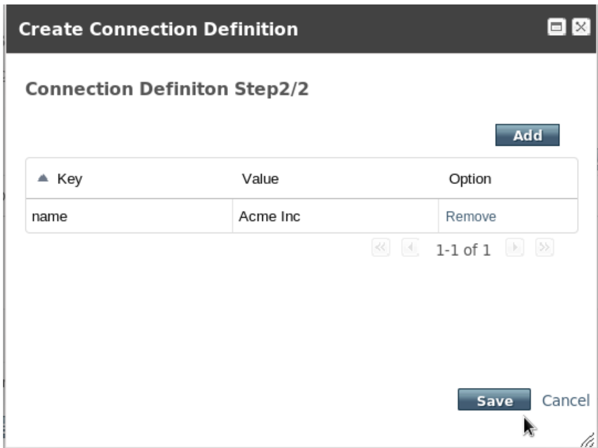
Figure 17.19. Create Connection Definition Property - Step 2
