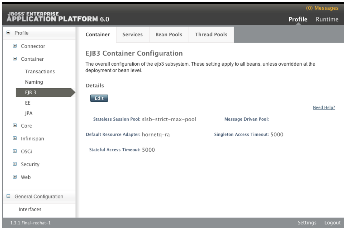
Figure 16.10. EJB3 Container Configuration panel in the Management Console (Standalone Server)
