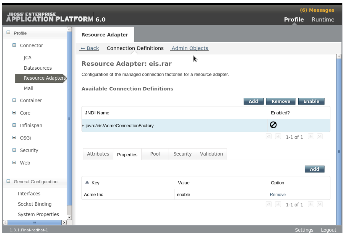
Figure 17.20. Create Connection Definition - Disabled
