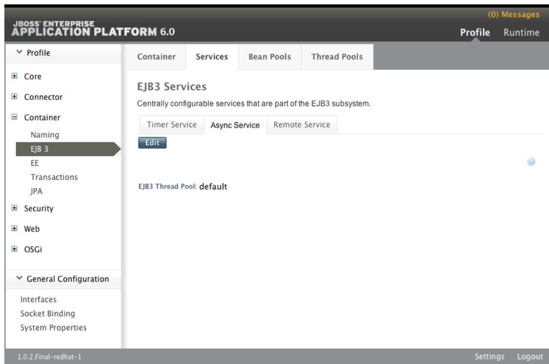
Figure 16.12. The Async Service tab of the EJB3 Services panel
