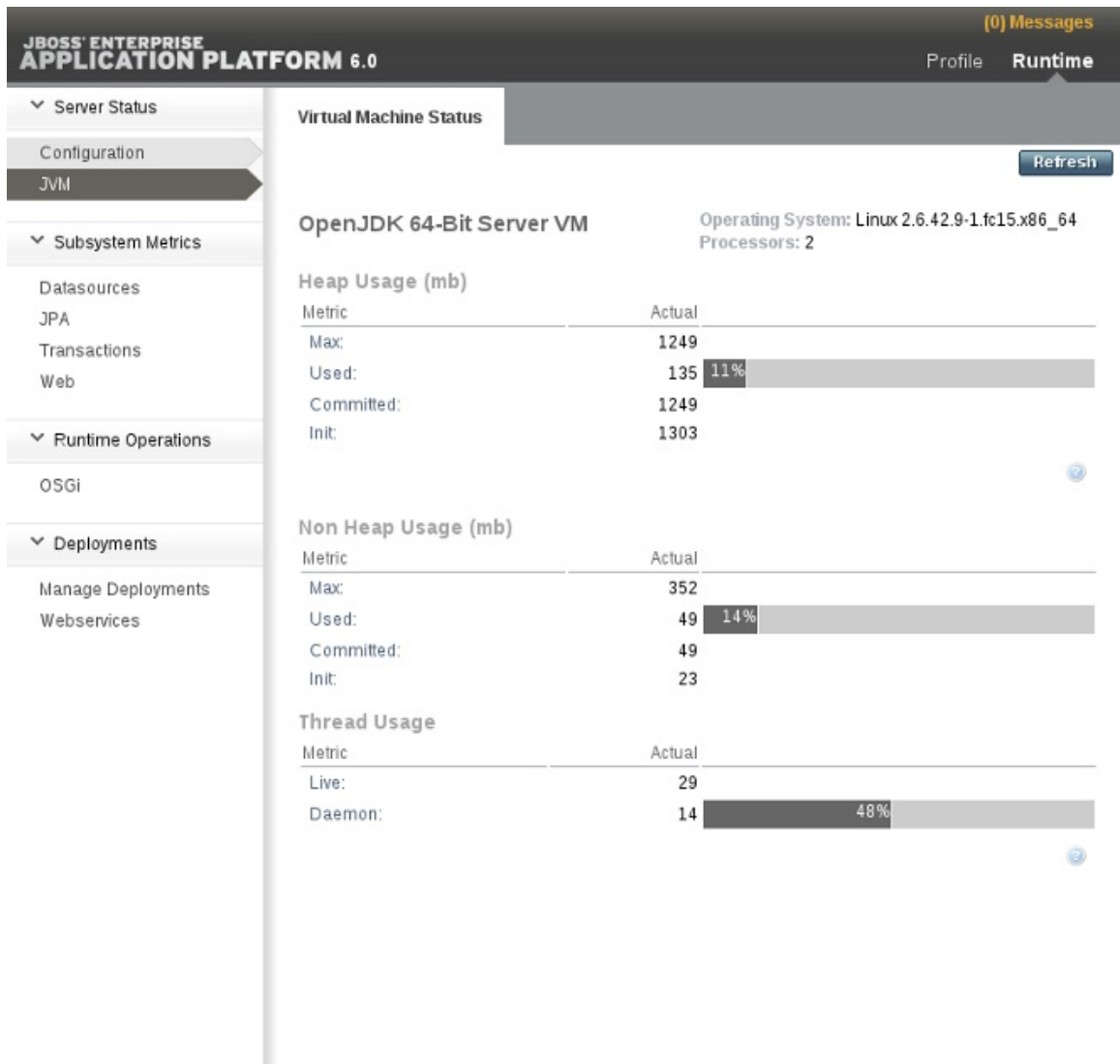
Figure 12.1. JVM status for a standalone server instance
