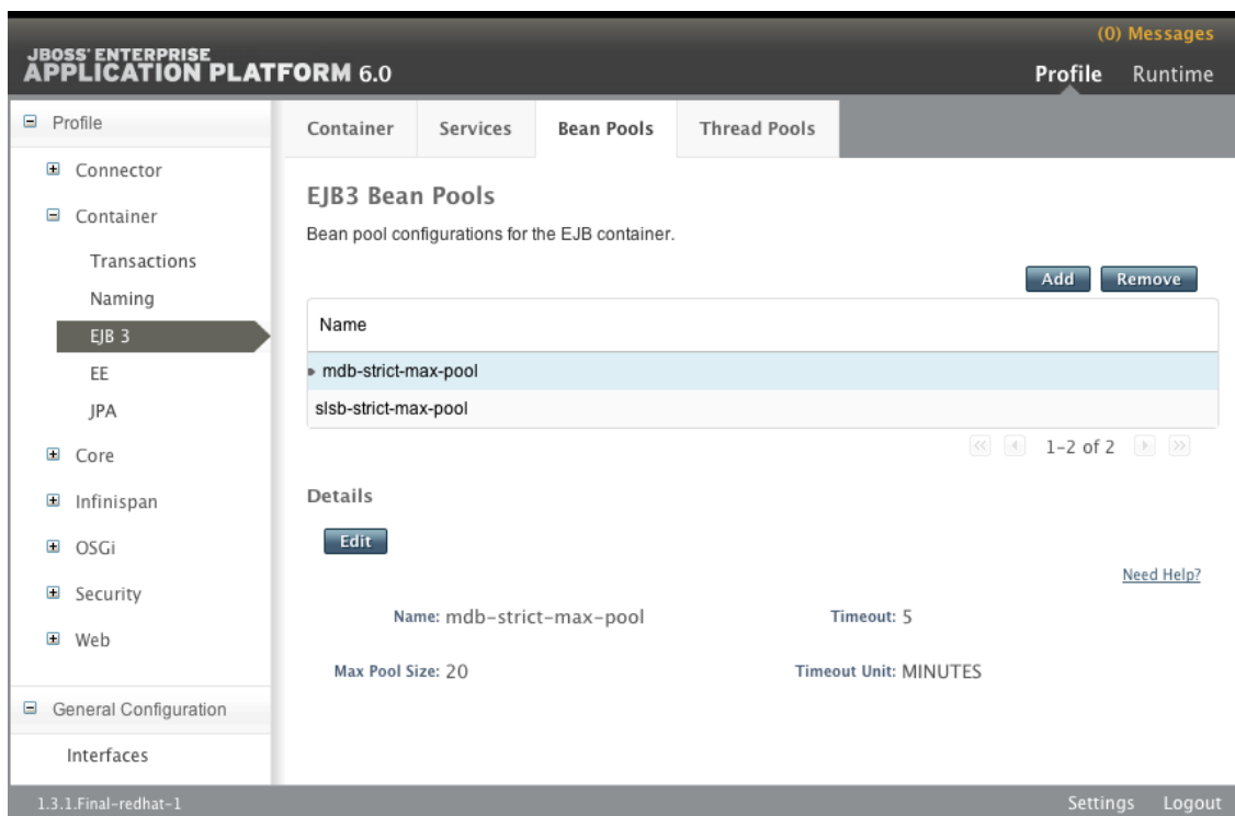
Figure 16.4. EJB3 Bean Pools Panel
