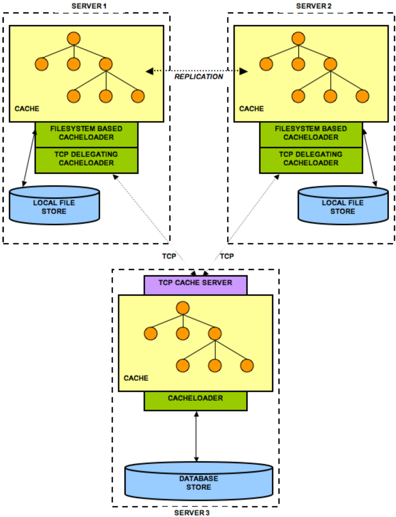
Figure 9.6. Multiple cache loaders in a chain
