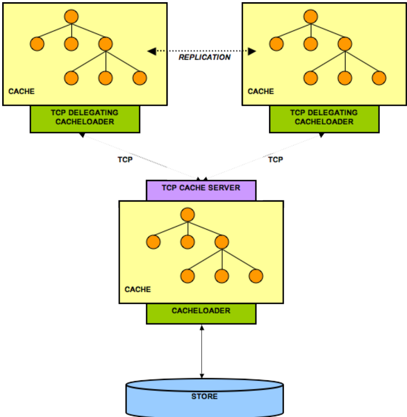
Figure 9.5. TCP delegating cache loader
