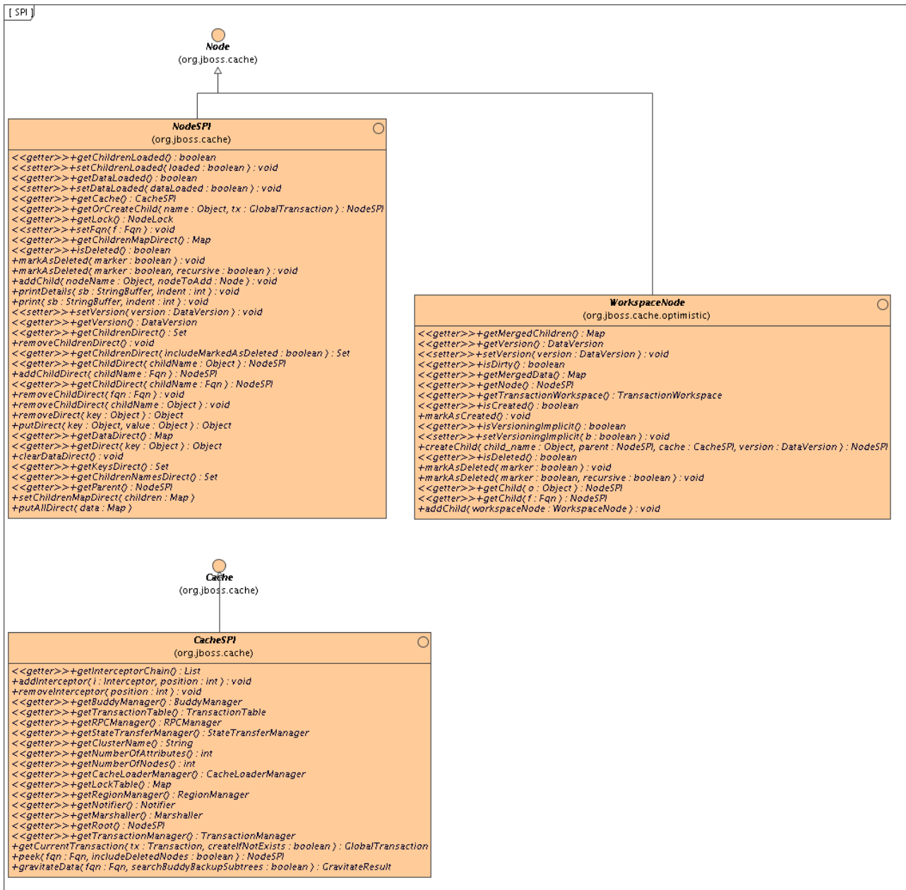
Figure 7.2. SPI Interfaces
