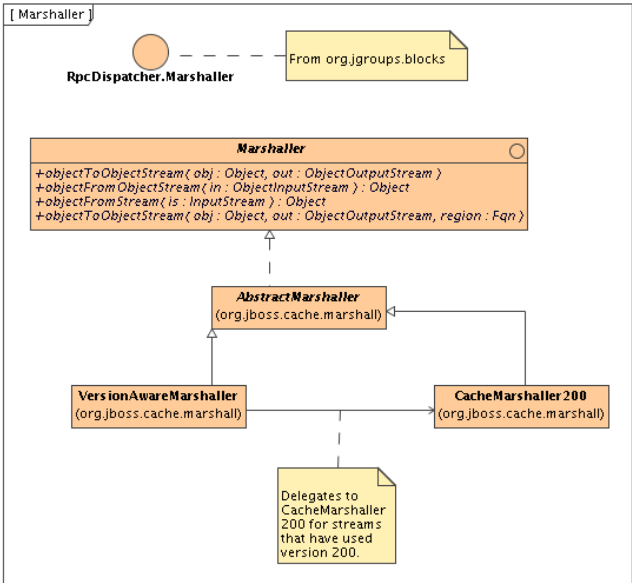
Figure 7.3. The Marshaler interface
