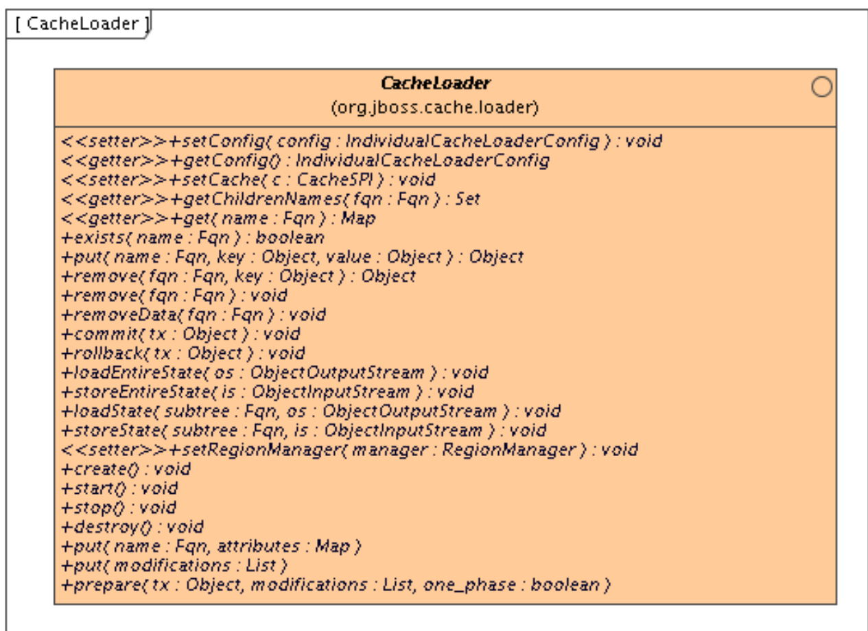
Figure 9.1. The CacheLoader interface
