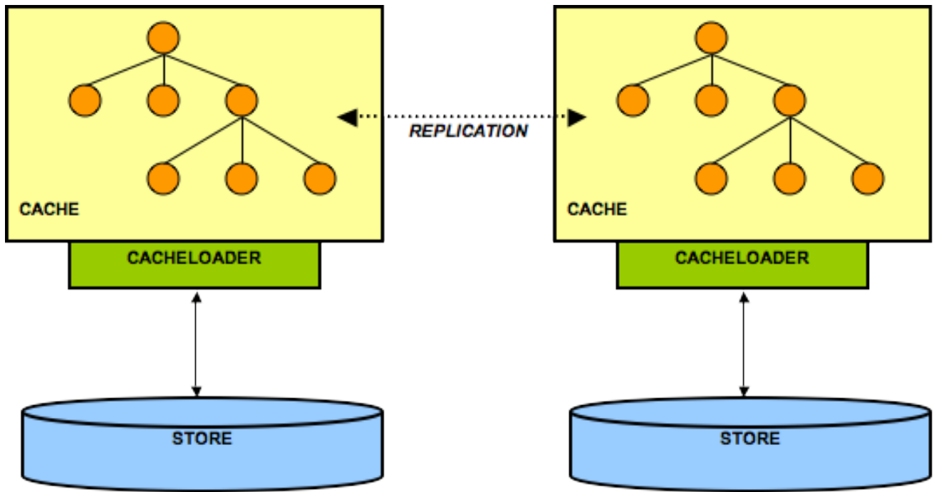
Figure 9.4. 2 nodes each having its own back end store
