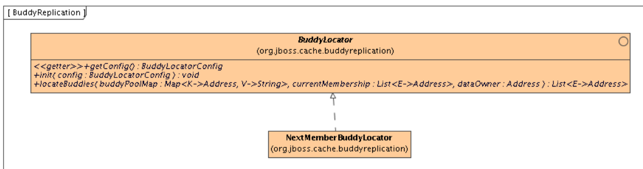
Figure 8.1. BuddyLocator
